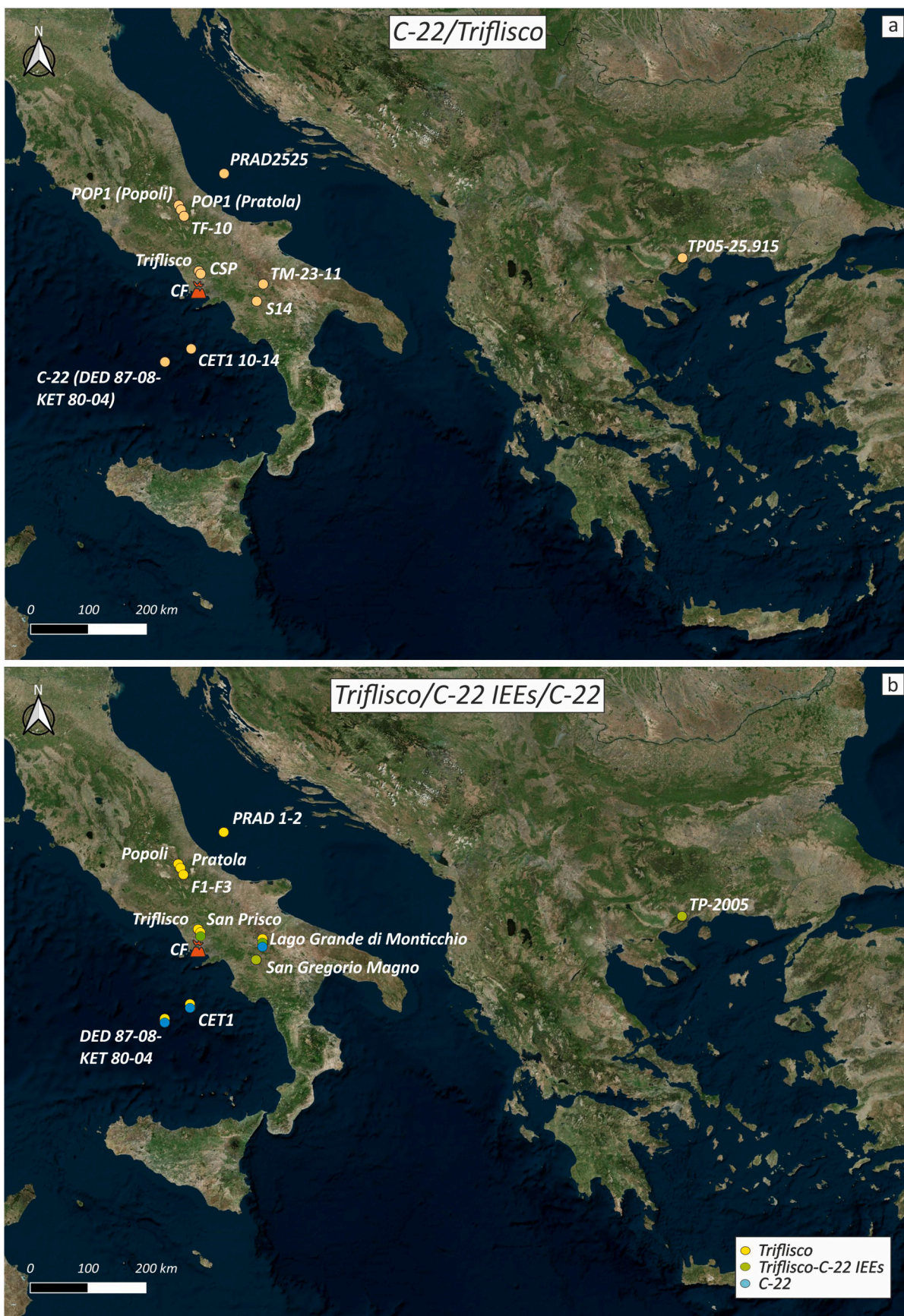
Fig. 13. a) Dispersal area of the C-22 eruption according to literature data; b) Dispersal area of the Triflisco (yellow dots), Triflisco-C-22 IEEs (green dots) and C-22 (sky-blue dots) according to the new correlations provided in this work.
