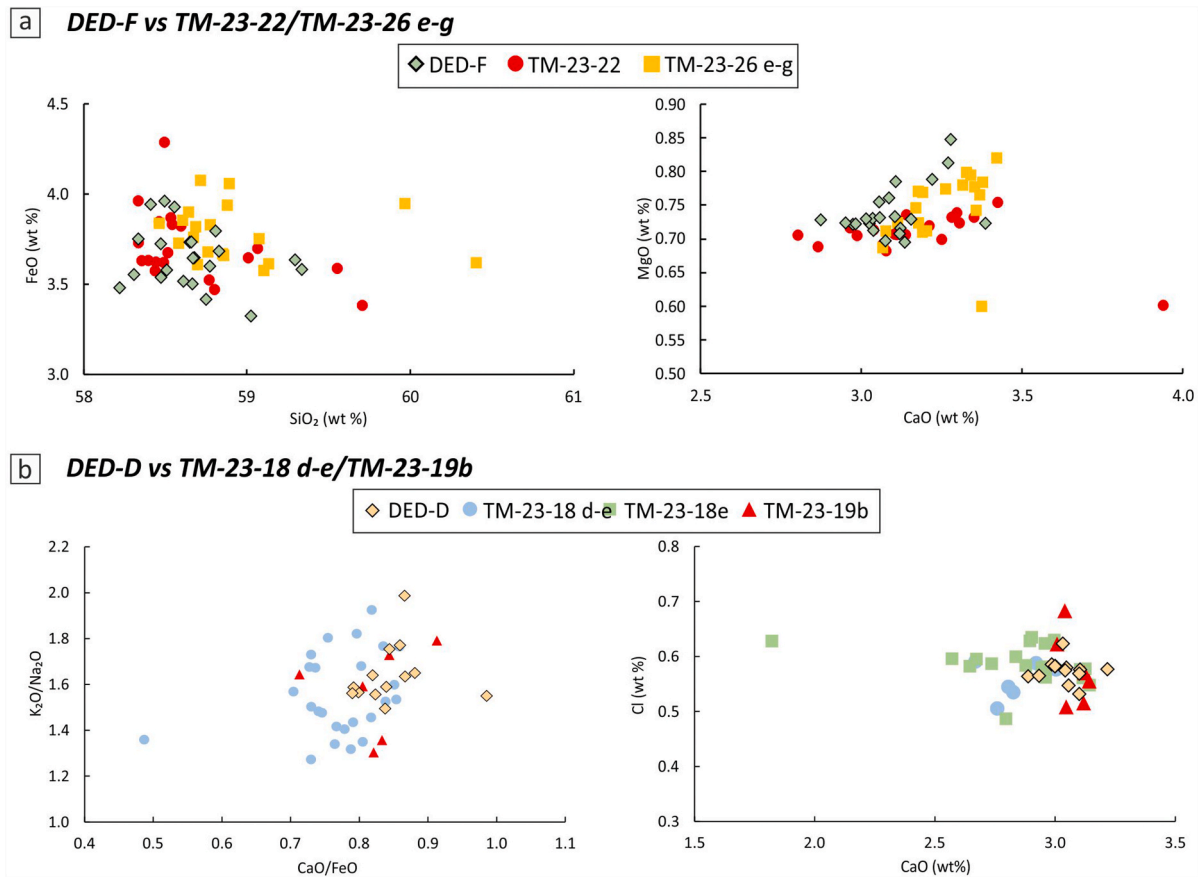
Fig. 7. Comparison between the investigated DED-F and DED-D and their equivalents. a) Major element composition of DED-F in comparison with the Monticchio tephras TM-23-22/TM-23-26-e-g (Wulf et al., 2004). b) Major element composition of DED-D in comparison with the Monticchio TM-23-18d-e/TM-23-19b (Wulf et al., 2004).
