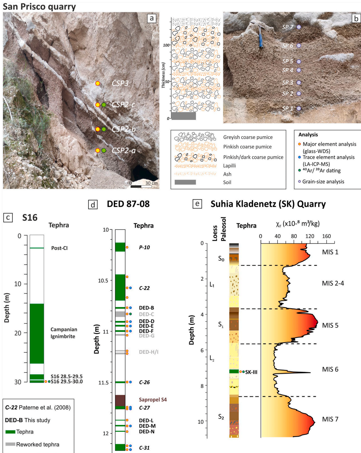
Fig. 2. a) and b) Photographs and stratigraphic log of the San Prisco sequence (41°05'31''N; 14°17'25''E, Campanian Plain; Fig. 1). a) CSP2 (a, b and c) and CSP3 were sampled for EMPA and 40 Ar/ 39 Ar analyses. b) Samples SP1 to SP7 were sampled for grain-size analyses. Full dataset is provided in the Supplementary Material (S1 and S3). c) Simplified section of the core S16 (41°07'02''N; 14°01'23''E, Campanian Plain) investigated for the first time in this study; d) Simplified section of the marine core DED 87-08 (39°42'14''N; 13°34'93''E, Central Tyrrhenian Sea); e) Loess-paleosol succession of the Suhia Kladenetz Quarry (43°27'24.0''N, 24°41'26.7''E; Central North Bulgaria, Lower Danube). For further details about the core DED 87-08 and Suhia Kladenetz Quarry successions the reader is referred to Paterne et al. (1988, 2008) and Jordanova et al. (2022), respectively.
