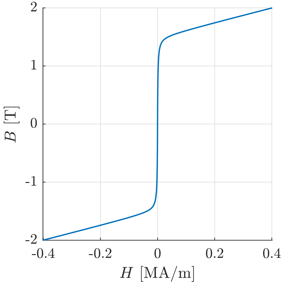
Figure 4: The constitutive relation for the magnetic field in the CM particles.
