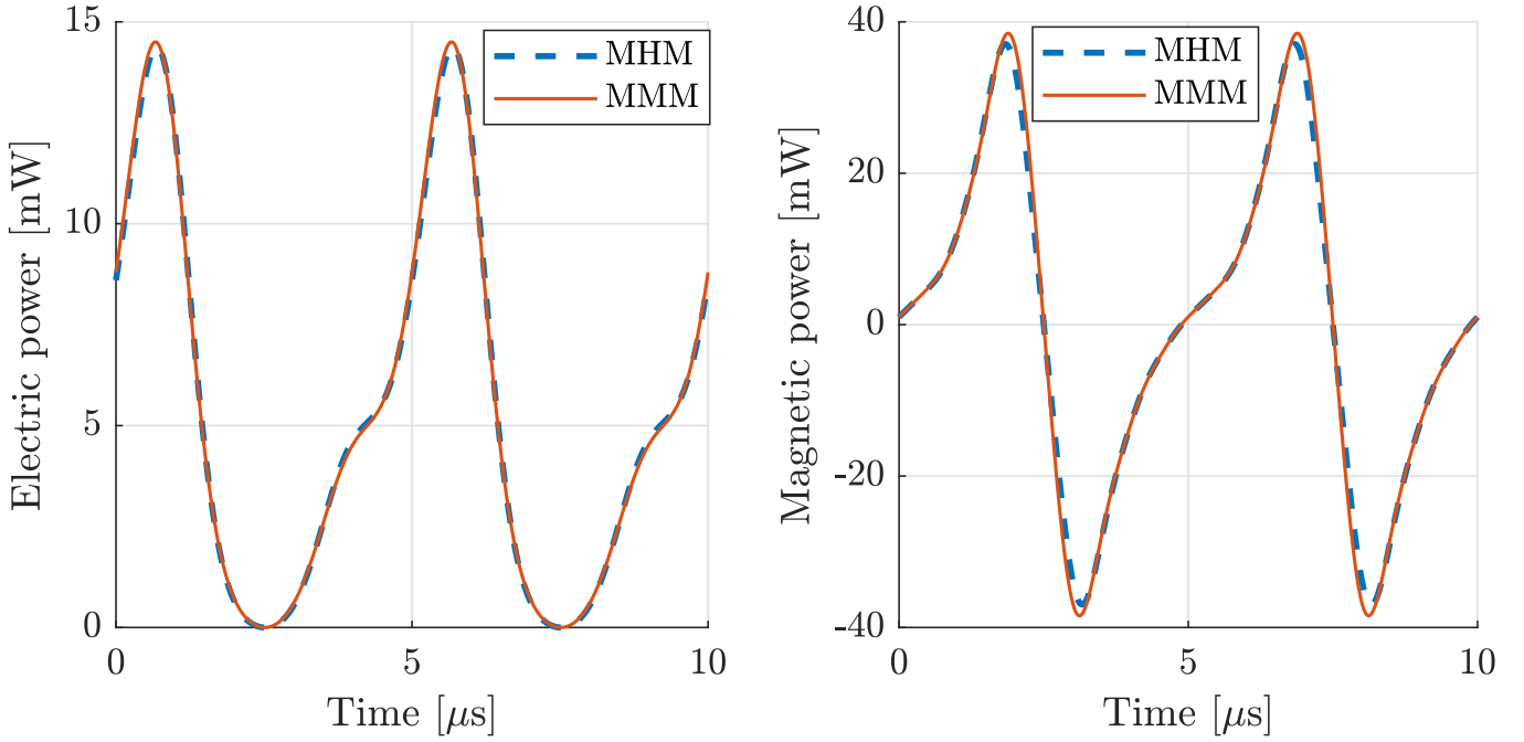
Figure 9: Comparison between MHM and MMM in the electric (left) -and magnetic (right) power.
