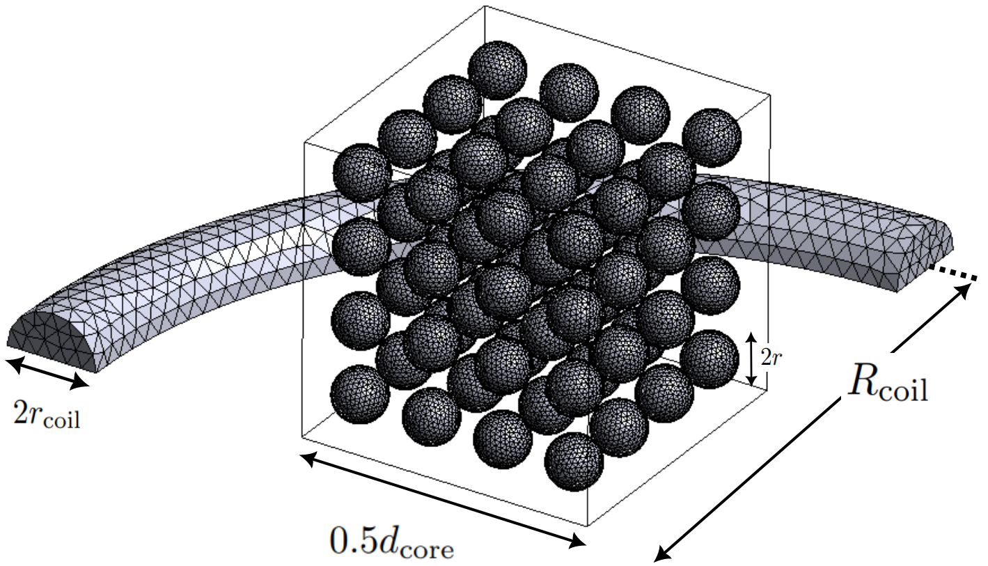
Figure 1: The original modelling domain consists of a coil, and the composite material made of conducting nonlinear magnetic particles. Due to symmetry, in the simulations only the one-eighth of the full geometry, shown in the figure, is modelled.
