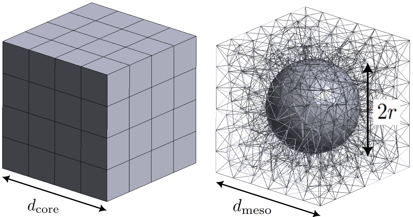
Figure 2: Left: the homogenized macro-scale CM domain of the original problem. Right: the meso-scale cell representing the CM.
