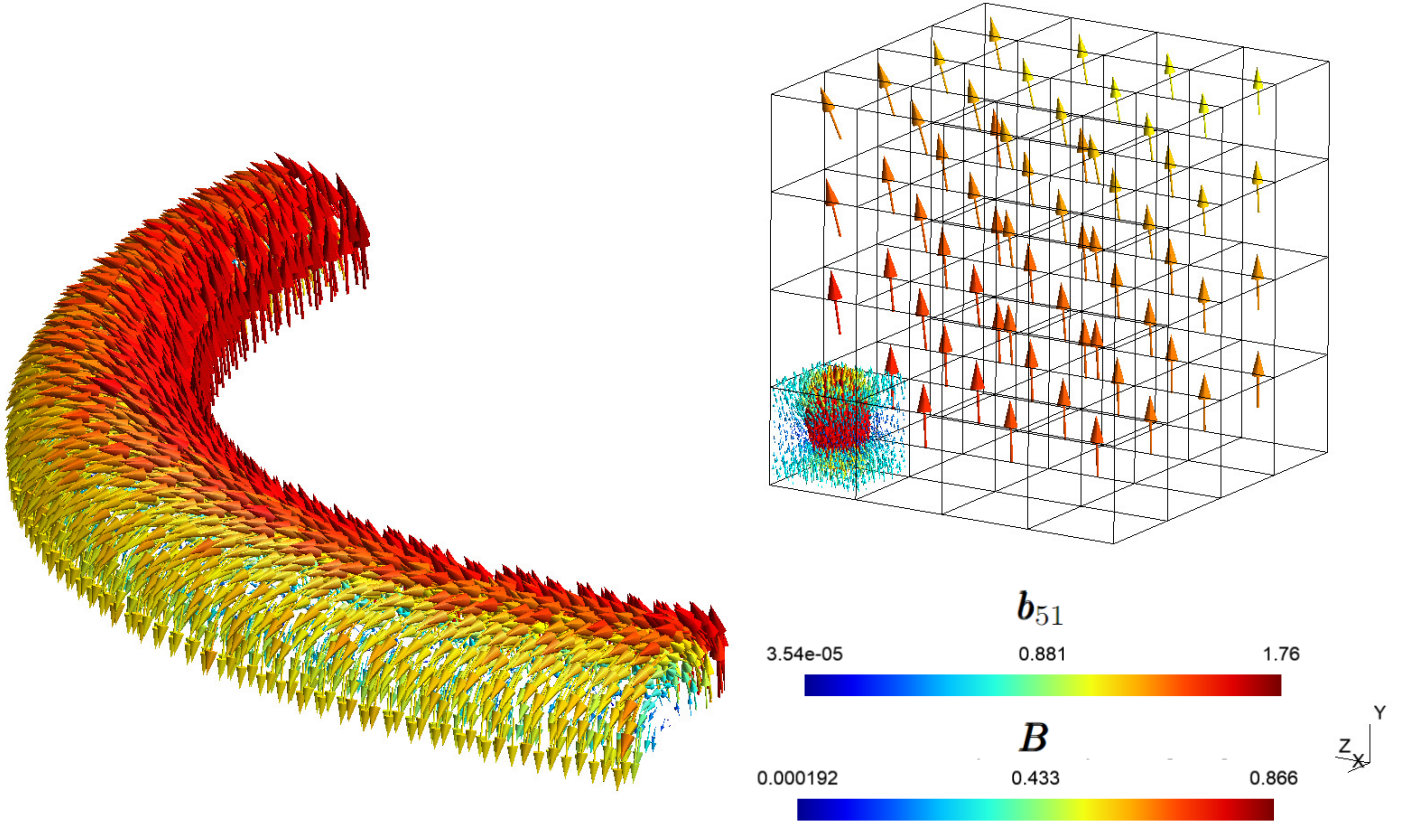
Figure 11: Macroscale magnetic flux density in the coil and the composite material. In addition, mesoscale \mathbf{b} is merged into the corner element of the homogenized core domain.
