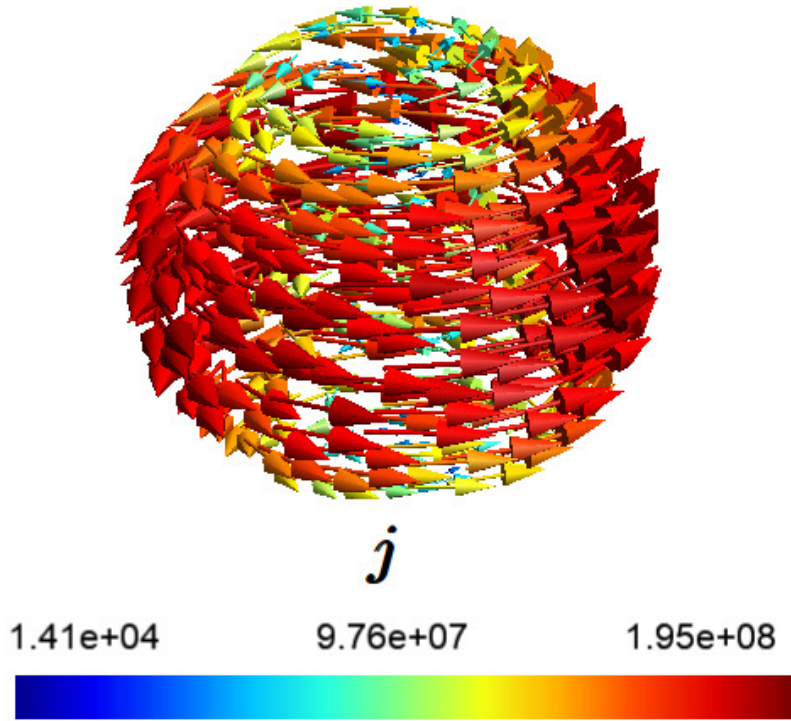
Figure 7: Electric current density in the cell when sourced with y-directional B(t) = 0.8 \cdot \sin(\omega t) [T] at the frequency of 100 kHz.
