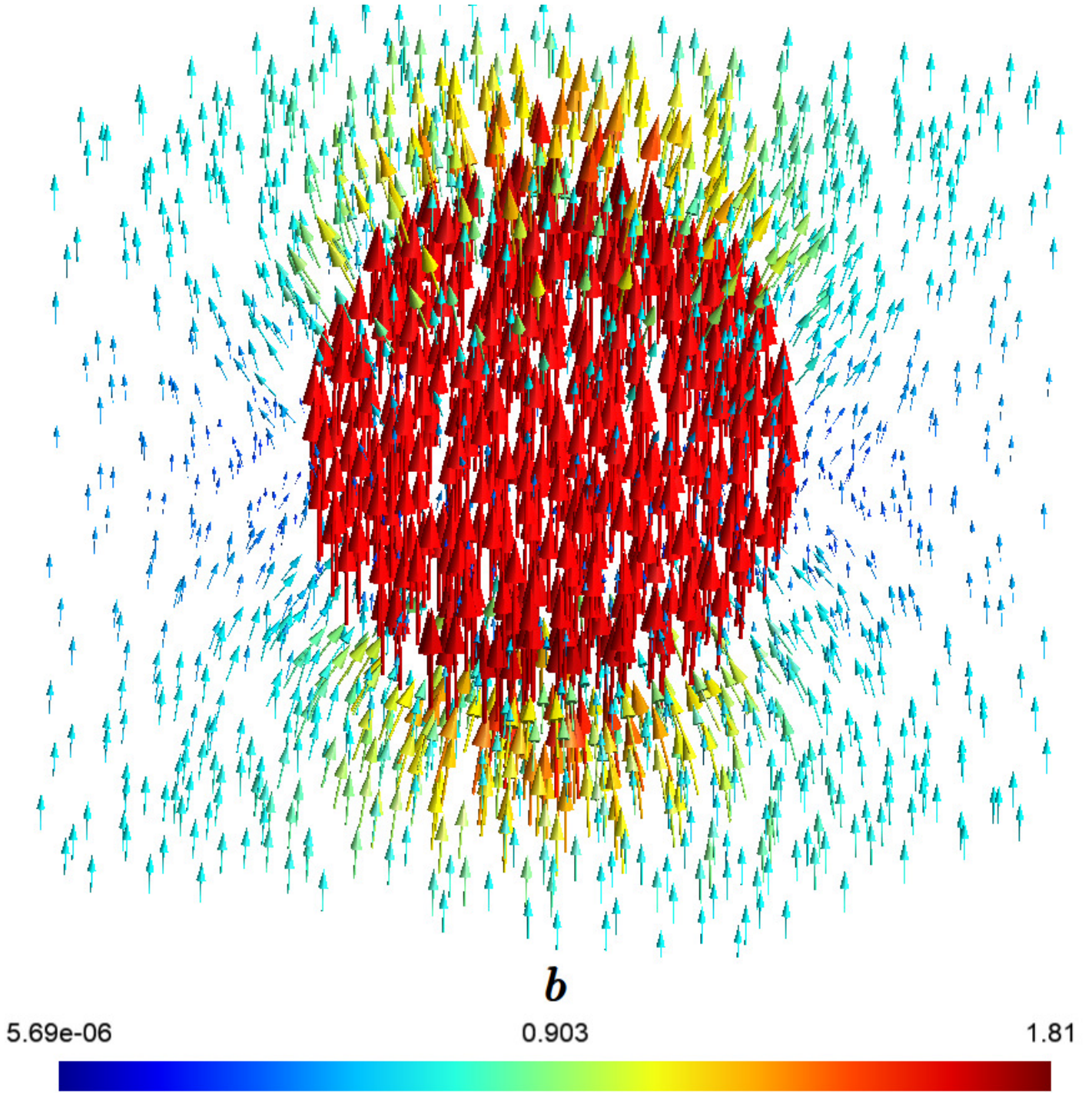
Figure 6: Magnetic flux density in the cell when sourced with y -directional B(t) = 0.8 \cdot \sin(\omega t) [T] at the frequency of 100 kHz.
