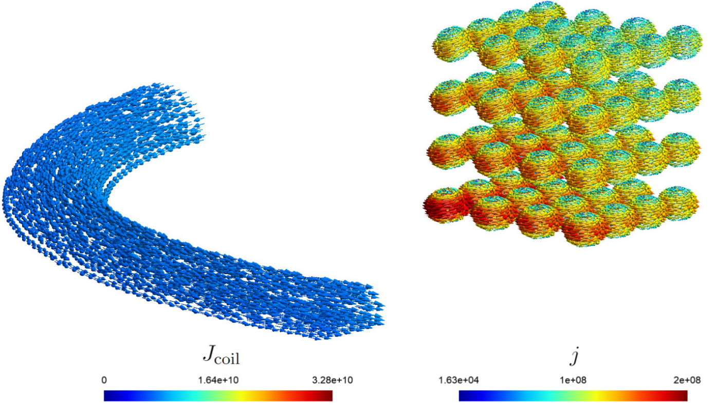
Figure 10: In-time varying macroscale current density in the coil (left) induces eddy currents in the mesoscale particles (right).
