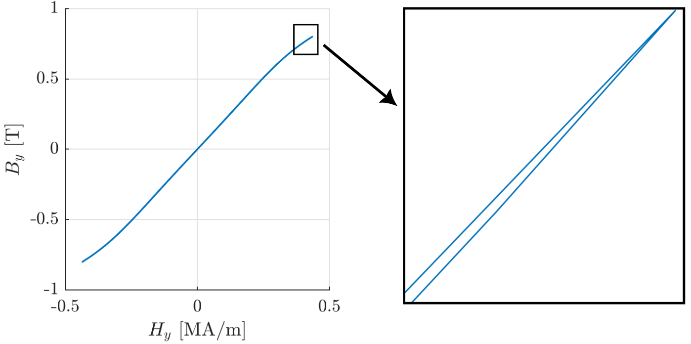
Figure 5: The homogenized \mathbf{B} - \mathbf{H} relation (left) has dynamic hysteresis due to the induced eddy currents in the particle of the cell as shown in the close-up figure on the right.
