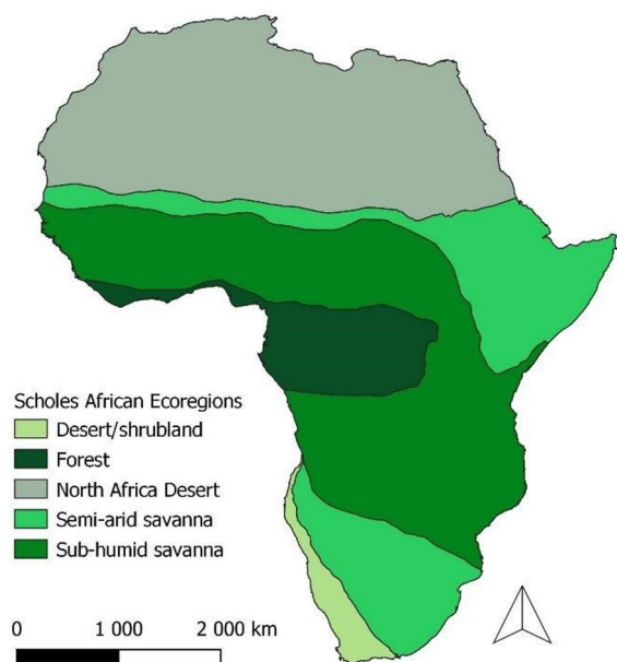
Figure 1. The Scholes African Ecoregions Map (Ernst & Scholes, 2023) was delineated by regrouping and smoothing the vegetation classification of the UNESCO/AETFAT/UNSO (White's) Vegetation Map of Africa (White, 1983) in accordance with the delineations of the distributions of Mean Annual Precipitation-determined ("stable") and Disturbance-determined ("unstable") savannas in Africa by Sankaran et al. (2005).
