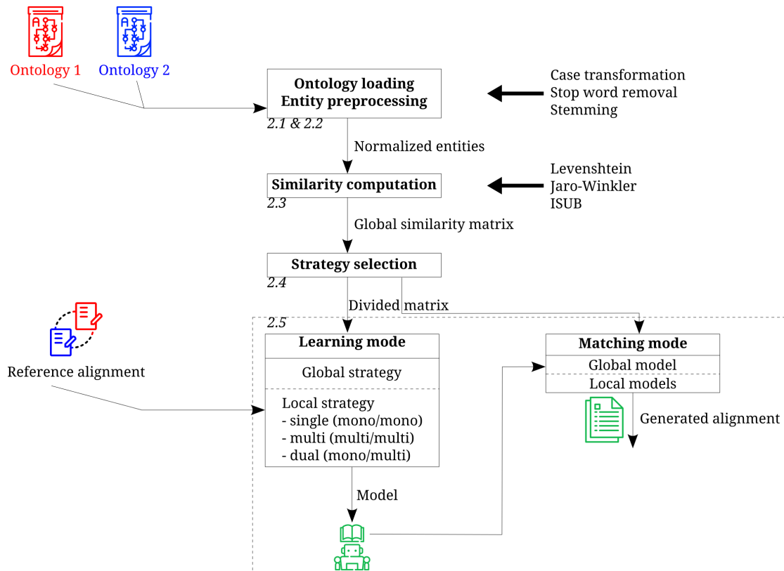
Figure 1: System workflow
