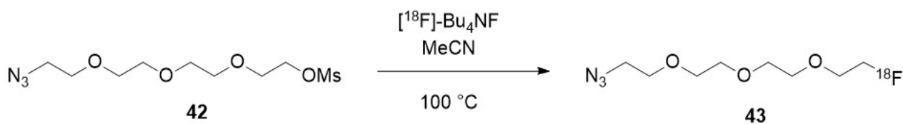
Figure 28. Synthesis of [ ^{18}\text{F} ]-fluoroethyl-diethyleneglycol-ethylazide 43 .
