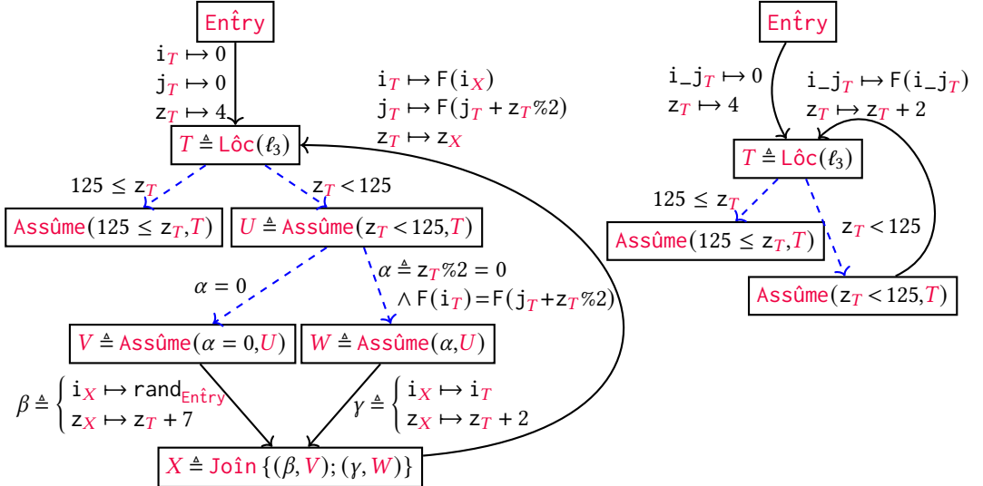
(c) Analysis with bare SSA translation (left: \text{Lift}(\widehat{\text{FA}}) , Sections 6 and 7), and translation combined with numerical analysis and simple rewrites (right: \text{Lift}(\widehat{\mathcal{Q}}(\widehat{\text{FA}}\widehat{\times}\widehat{\mathbb{N}})) ). For legibility, we use T, U, V, W, X as short names for terms and \alpha, \beta, \gamma as short names for edges
