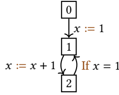
Fig. 14. Example of non-convergence for non-monotone programs
