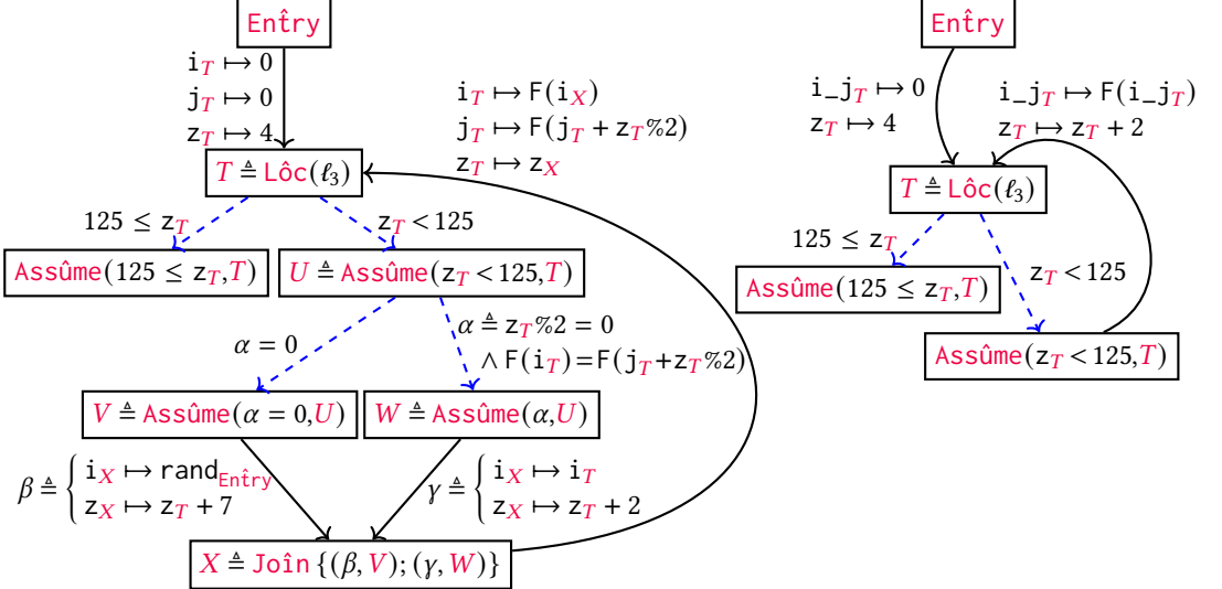
(c) Analysis with bare SSA translation (left: Lift(FA), Sections 6 and 7), and translation combined with numerical analysis and simple rewrites (right: Lift(Q̂(FAxN))). For legibility, we use T, U, V, W, X as short names for terms and \alpha, \beta, \gamma as short names for edges
