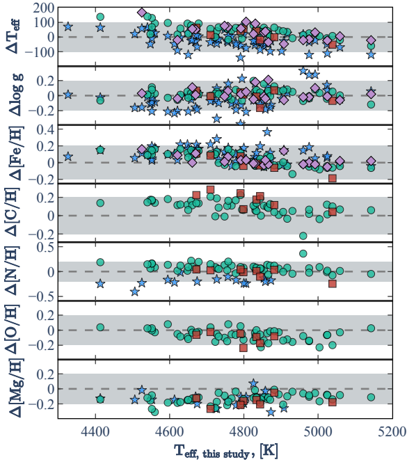
Fig. 6. Differences between [X/H] , \log g , and T_{\text{eff}} coming from the literature and derived in this study. The comparisons are done using the Gaia DR3 (blue stars), APOGEE DR17 (green circles), LAMOST DR7 (orange squares), and PASTEL (purple diamonds) catalogues. The shaded regions indicate \pm 0.2 dex and \pm 100 K.
