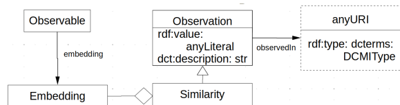
Figure 5: Distributional similarity in OntoLex-FrAC
