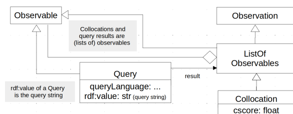
Figure 7: Proposed query extension
