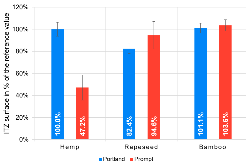
Figure 7. Comparison of mean halo surface between Portland and Prompt binders. Hemp in Portland cement as reference.
