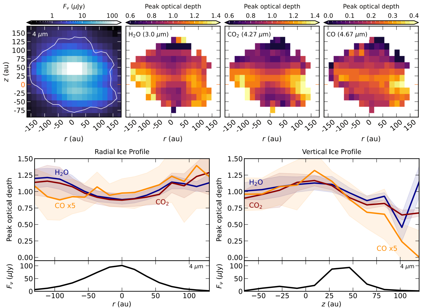
Fig. 4: Overview of the variations in the relative strength of the three strongest ice features, H 2 O, CO 2 , and CO.
