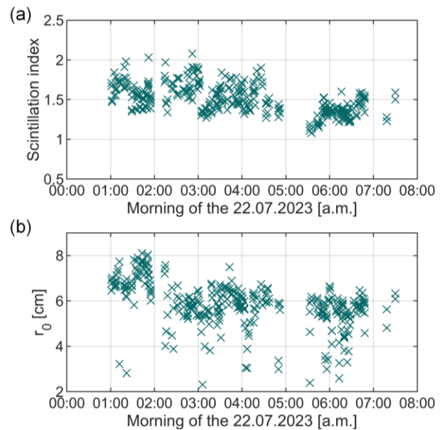
Fig. 10. Measured Scintillation Index as well as Fried's coherence length r_0 over the measurement time horizon.
