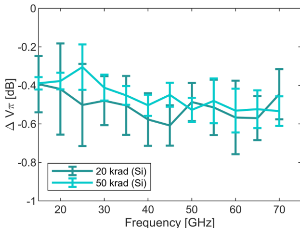
Fig. 9. Change in V_\pi over frequency after different TID. Unpackaged and unpassivated plasmonic modulators were exposed to a TID of 20 or 50 krad (Si). Later the difference in electro optic modulation efficiency was measured. A dose independent reduction around 0.5 dB was measured.
