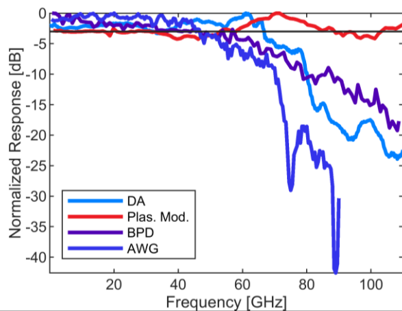
Fig. 4 Measured bandwidth of individual components of the communication system. Driving amplifier (DA), plasmonic modulator (Plas. Mod.), balanced photodetectors (BPD) as well as arbitrary waveform generator (AWG) are shown. The packaged Plasmonic modulator exhibits a 3 dB bandwidth in excess of 110 GHz.
