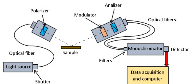
Fig. 1. The experimental set-up used in ellipsometry measurements
