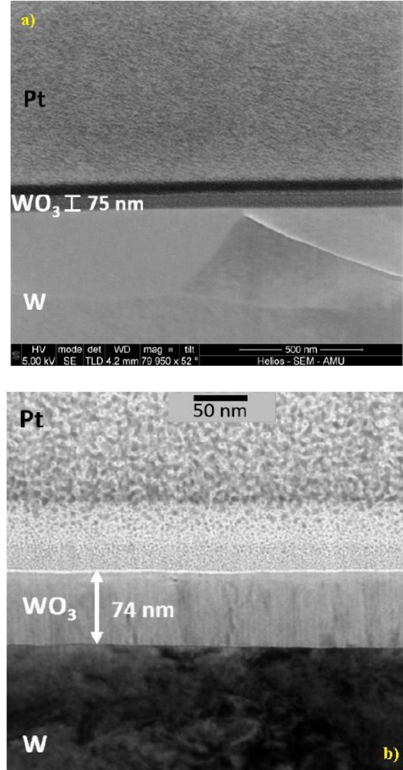
Fig. 3. a) SEM image of unexposed \text{WO}_3 sample (S4) and b) TEM image of room temperature He plasma exposed \text{WO}_3 (S5), prepared by FIB cross-section [21]
