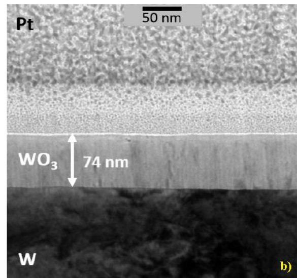
Fig. 3. a) SEM image of unexposed WO_3 sample (S4) and b) TEM image of room temperature He plasma exposed WO_3 (S5), prepared by FIB cross-section [21]
