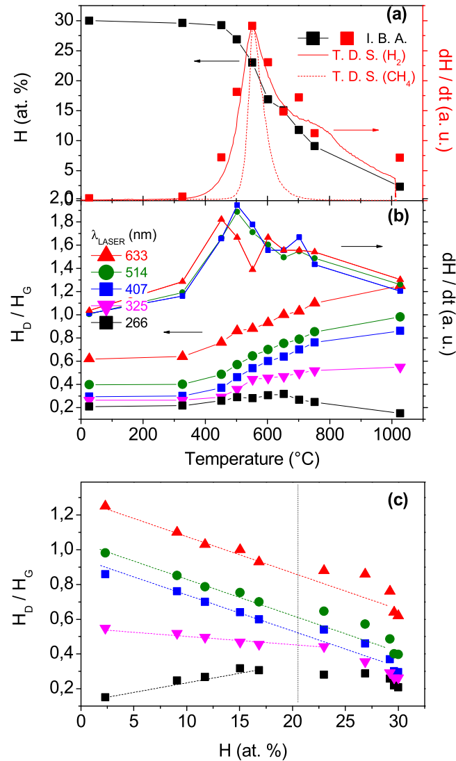
Figure 10. Hydrogen content evolution under post deposition heat treatment. (a) Ion beam and TDS. (b) D over G band relative intensity ratio evolution and its derivative with temperature. (c) H_D/H_G and H content correlation. Data of figure (a) is from [58]. Data of figures (b), (c) is from [48].
