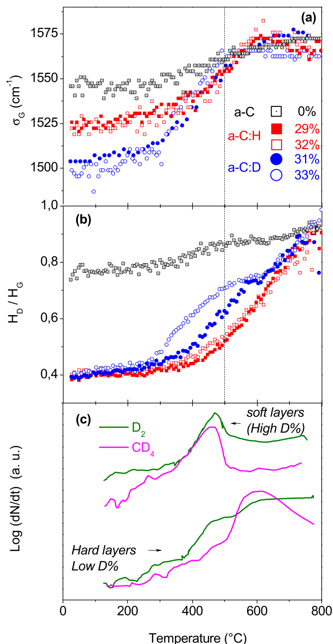
Figure 9. Band position and relative intensity ratio for amorphous hydrogenated and deuterated carbons. (a) G band position (carbon stretching). (b) D over G band intensity ratio. (c) Thermal desorption spectra of soft and hard samples. Data of figure (a) and (b) are from [81]. Data of figure (c) are from [82]. Laser wavelength used was 514 nm.
