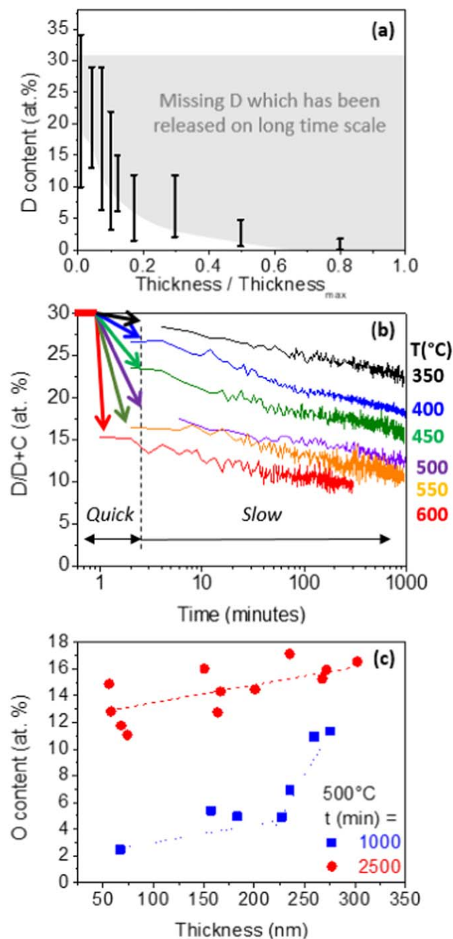
Figure 11. Slow deuterium release during backing. (a) D content decrease in Tore Supra deposits, adapted from [105, 106]. (b) D content evolution deduced from the Raman spectra in laboratory samples. (c) In depth oxygen content evolution at 500 °C with various heating time for a laboratory sample. Data of figure (a) are from [105, 106]. Data of figure (b) are from [81, 107]. Data of figure (c) are from [48].
