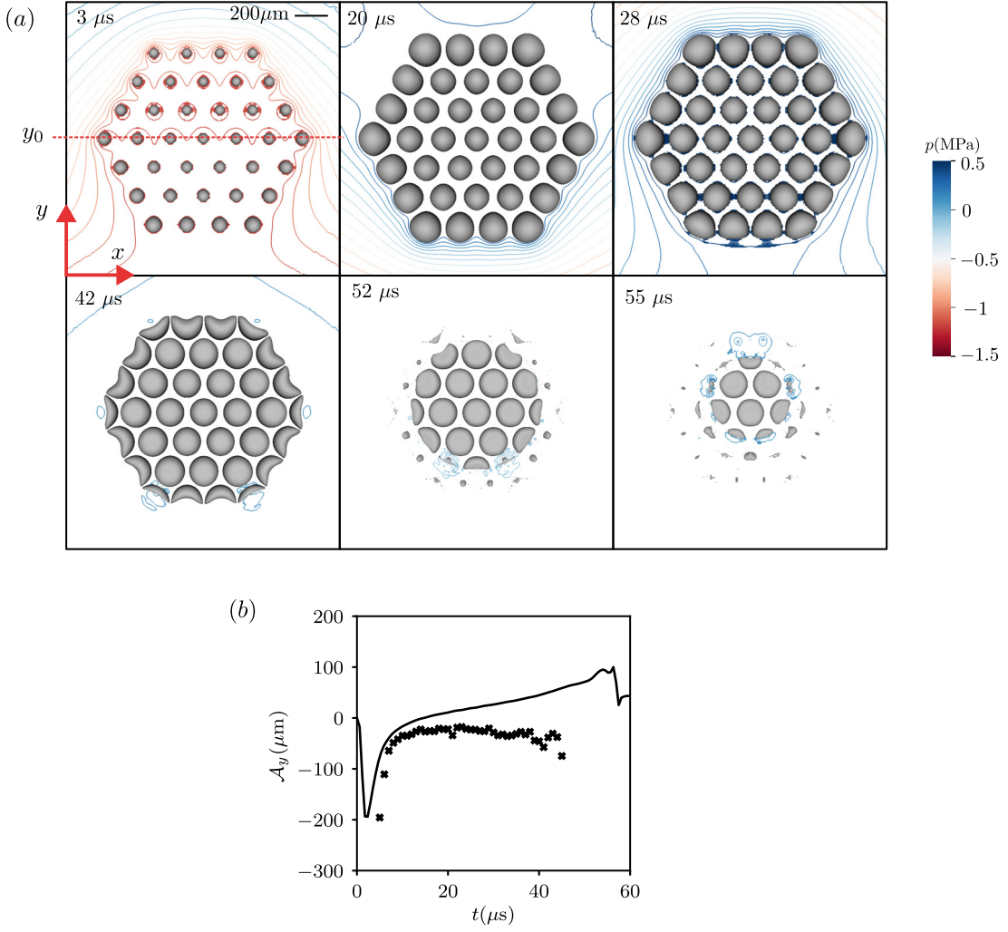
FIG. 8. (a) Top view of the cluster of 37 bubbles in a hexagonal arrangement expanding from 20 \mu\text{m} hemispherical nuclei. The effective speed of sound in the liquid is 1480 m/s. Isobars are shown with a colormap. (b) The evolution of the asymmetry parameter A_y(t) obtained from the numerical simulations (solid line) and the experiments (crosses).
