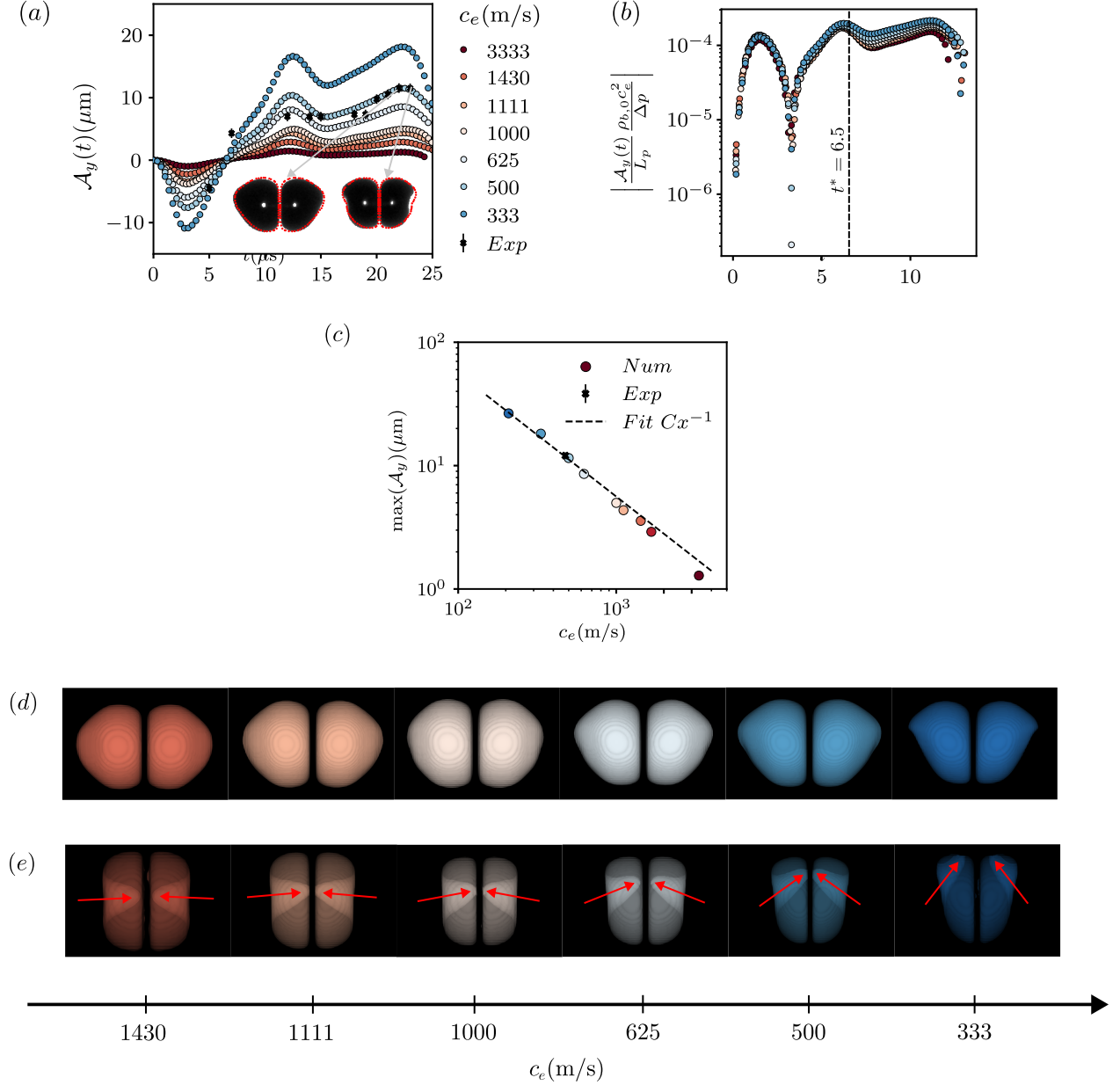
FIG. 5. Effect of the effective speed of sound on the asymmetry for the particular case where the bubbles are nucleating from a pair of hemispherical nuclei with radii of 20 \mu\text{m} each, and separated by a distance d = 200 \mu\text{m} . (a) The time evolution of \mathcal{A}_y is shown for different values of the effective speed of sound (colormap), alongside the experimentally obtained values (black crosses). The experimental bubble shapes overlaid with their numerical counterparts (red dots) at t = 22 and 23 \mu\text{s} are illustrated in the inset. (b) The evolution of the dimensionless \mathcal{A}_y(t) as a function of dimensionless time ( t^* = tU_c/R_0 ) obtained using the scaling predicted from Eq. (12) for different values of c_e . (c) The maximum value of the asymmetry parameter \max(\mathcal{A}_y) is plotted on a log-log scale as function of the effective speed of sound along with the experimental point where its c_e is obtained by matching \max(\mathcal{A}_y) with the numerical data. A fit of all data (dashed line) is also plotted to demonstrate that \max(\mathcal{A}_y) decays like c_e^{-1} as predicted by Eq. (12) for given T_p . (d) The bubble shapes at the instant of \max(\mathcal{A}_y) are shown for different effective speeds of sound in the liquid. (e) Semitransparent bubble shapes are shown to visualize the jet generated during the last stages of collapse, whose direction is highlighted with red arrows.
