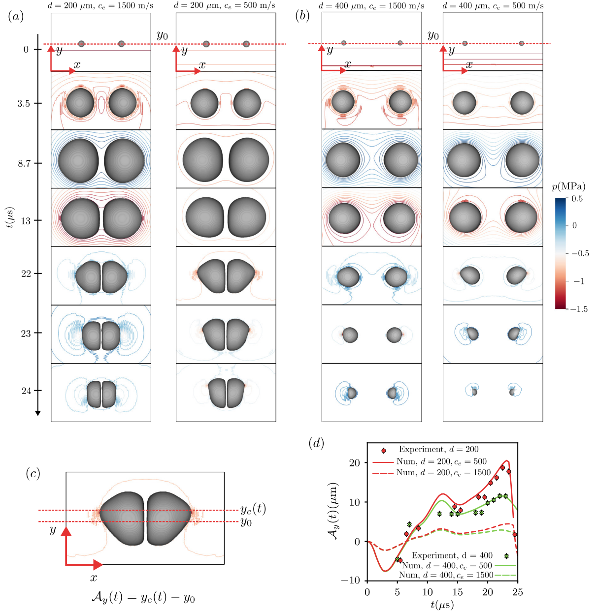
FIG. 4. Comparison of the numerical results for two different values of the effective speed of sound, i.e. c_e = 1500 \text{ m/s} and c_e = 500 \text{ m/s} . The bubble pair evolves from hemispherical nuclei with radii of 20 \mu\text{m} . In (a) and (b), the top view of the bubble shape and pressure field are displayed at subsequent times shown. (a) Separation distance d = 200 \mu\text{m} between the nuclei with c_e = 1500 \text{ m/s} on the left and c_e = 500 \text{ m/s} on the right. (b) Separation distance d = 400 \mu\text{m} between the nuclei with c_e = 1500 \text{ m/s} on left and c_e = 500 \text{ m/s} on right. (c) A particular snapshot showing the definition of the asymmetry parameter \mathcal{A}_y(t) , which is defined as the shift of the bubble centroid in the y direction. (d) The time evolution of \mathcal{A}_y(t) obtained from the numerical simulations for all the cases discussed in (a) and (b) along with a comparison with experimental data. The error bars are equal to one pixel size ( 1.53 \mu\text{m} ) in the experiment snapshots.
