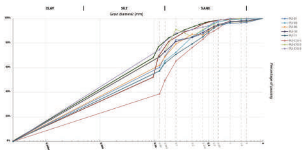
Figure 6: Superposition of the granulometric curves of Saïte 1 group, clayed masses and sediments taken from swampy areas. © C. Venton, M. Crépy, MFTMP
