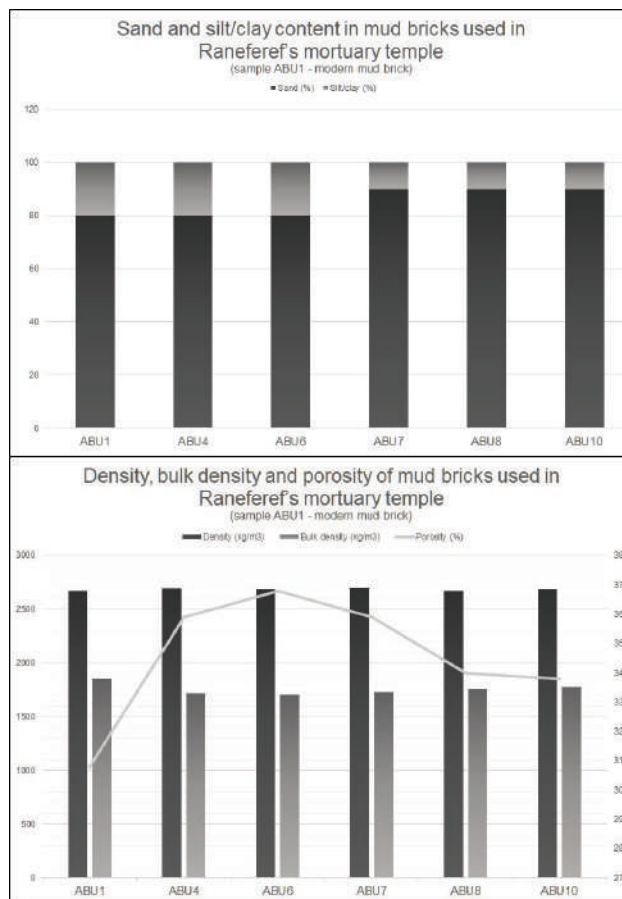
Figure 7: Material and physical aspects of mud bricks used in Raneferef's mortuary temple following results published by VANĚČEK (1993).
