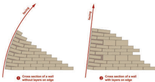
Figure 8: Use of bricks on edge in the masonry core, principle diagram. © M. Vanpeene
