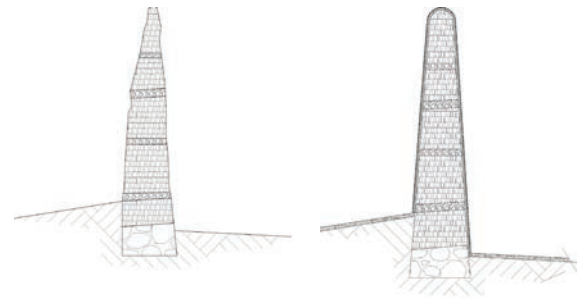
Figure 10: State of the cob wall before and after the restoration. © D. Gandreau et S. Moriset
