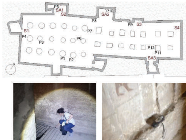
Figure 4: Layout of the tomb and location of the measurement points (S), painting location (P). © L. Joyanes Díaz
