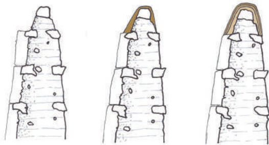
Figure 8: Realization of layers of sacrificial coatings, summit protection. © D. Gandreau et S. Moriset
