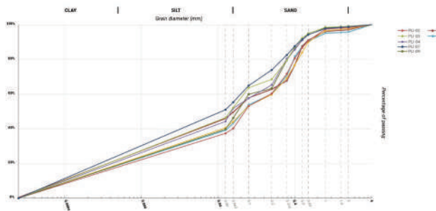
Figure 9: Superposition of the granulometric curves of the Saite 2 group and sediments from core sampling. © C. Venton, M. Crépy, MFTMP
