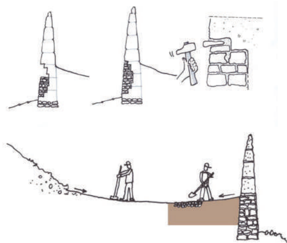
Figure 7: Realization of drainage slope and resumption of damage to the basement and the wall.
