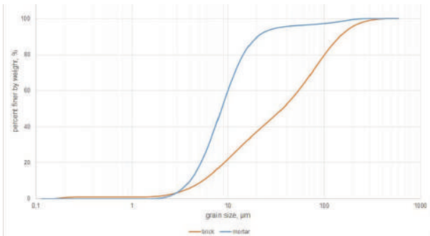
Figure 8: Fine-earth particle size distribution of tested brick and mortar.
