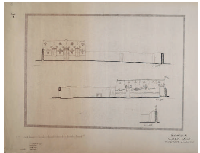
Figure 2: H. Fathy, Survey's of the Nubian area, Bayt Malik 'Abbas Aḥmad Ḥasbou, Kunuz Neighbourhood.
