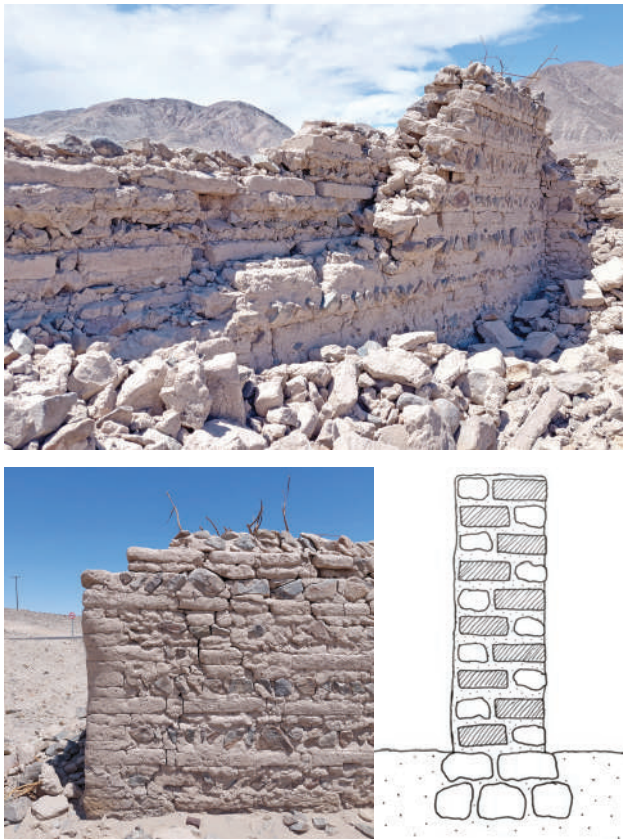
Figure 10: Construction system in the former Casablanca Hospital and Convent. a) and b) Views of walls c) Wall thickness diagram © Photographs and diagram by J. Quiroz Bravo, 2023
