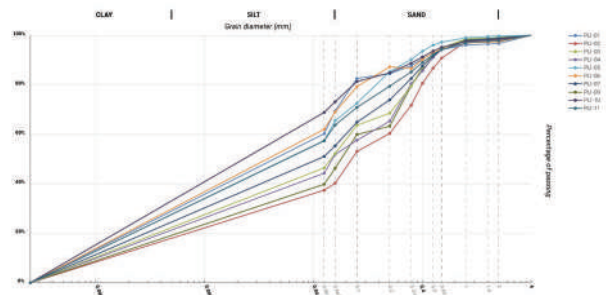
Figure 5: Granulometric curve of earth used in the Saite period. © C. Venton, M. Crépy, MFTMP
