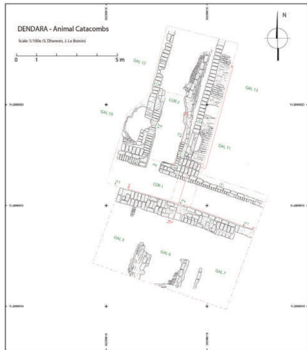
Figure 2: Top view of corridors 1 and 2. © S. Dhennin
