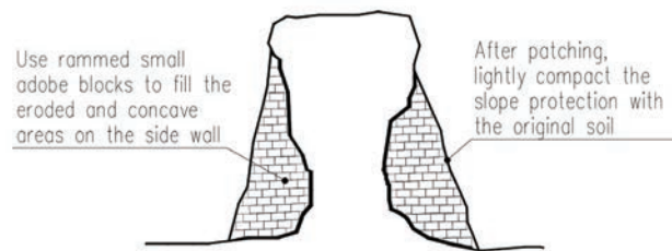
Figure 8: Reinforcement of the concave erosion Wall. © Y. Fan
