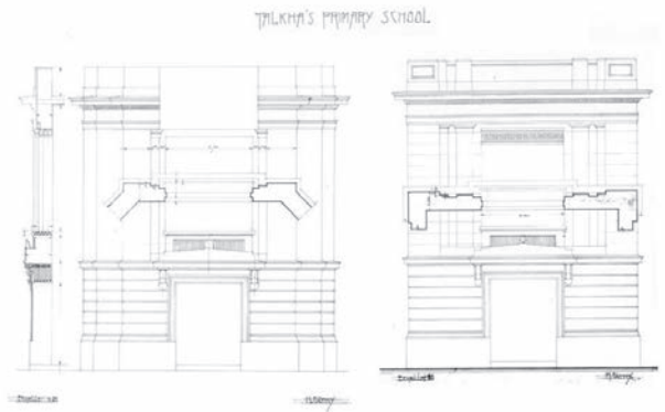
Figure 1: H. Fathy, Primary School, Talkha, 1928. © RBSC, The American University in Cairo
