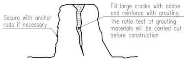
Figure 9: Reinforcement of the Cracked Wall. © Y. Fan
