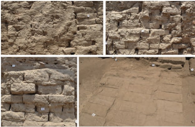
Figure 8: Mortar, bricks composition and size with details of the vertical and horizontal beds. © A. Altaher
