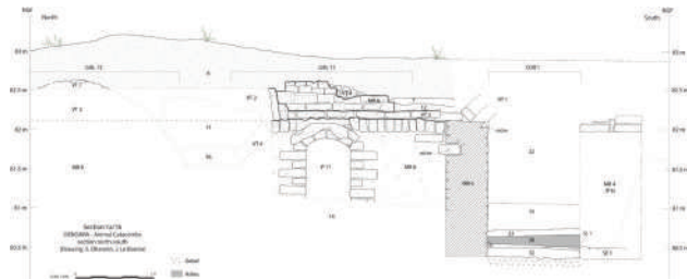
Figure 5: Section of corridor 1 and elevation of corridor 2. © S. Dhennin, J. Le Bomin
