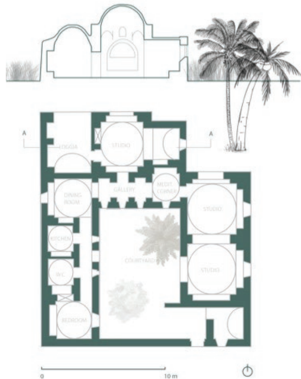
Figure 3: H. Fathy, Hamed Said House, 1945. Plan and section drawn from Fathy's archives in the RBSCL, The American University in Cairo. © Z. Bennouna
