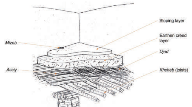
Figure 9: Ceiling system of the traditional construction building in the Ksar of Timimoun. © H. Ben Charif
