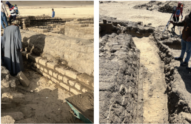
Figure 7: Two sections of the exterior corbeled wall, one left exposed and one encased in mud bricks.
