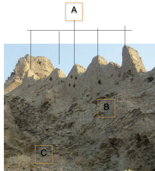
Figure 11: Detail of intervention for the part of the wall built in adobe. © S.M. Khalili
