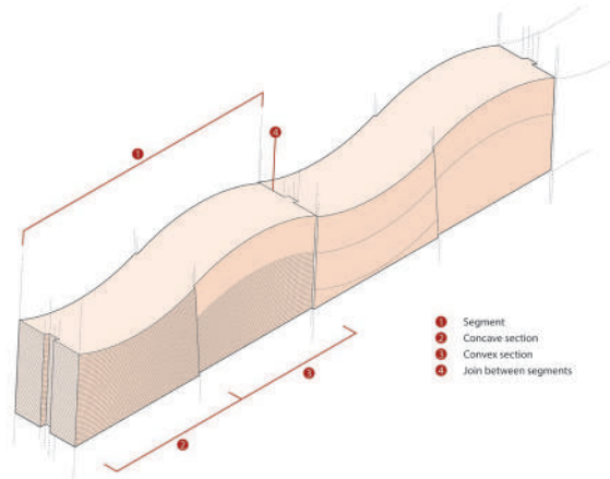
Figure 3: Walls with undulating courses, principle diagram. © M. Vanpeene
