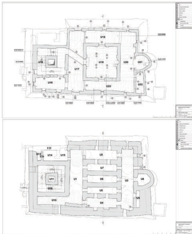
Figure 5: The plans of the mosque; the ground floor at the window level (below), the first floor (above).
