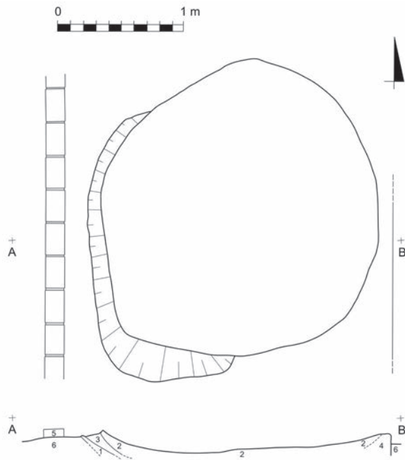
Figure 8: Mud brick workshop, plan and section (1-The first phase of the crust; 2-The second phase of the crust; 3-Sand fill with charcoals and pottery sherds; 4-Intact part of the enclosure wall of the pyramid courtyard; 5-Mud bricks; 6-Mud floor).
