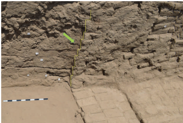
Figure 5: Wall's face slope, which produced by laid the bricks stepping each layer of bricks back slightly.
