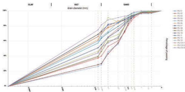
Figure 3: Granulometric curves for all the samples taken. © C. Venton, M. Crépy, MFTMP
