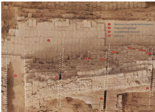
Figure 4: Extract of the photogrammetric survey of the wall after cleaning.
