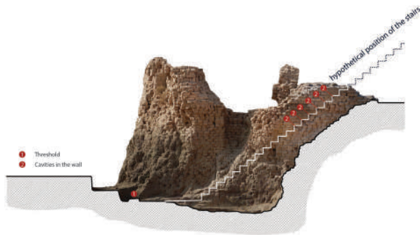
Figure 14: Reconstitution of the staircase. © M. Vanpeene
