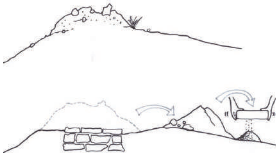
Figure 9: Restitution of the foundations. © D. Gandreau et S. Moriset
