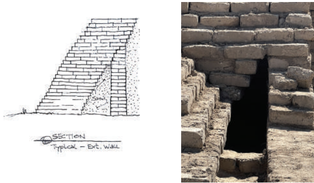
Figure 2: A field sketch of the corbeled exterior wall and the restored detail. © A. Crosby
