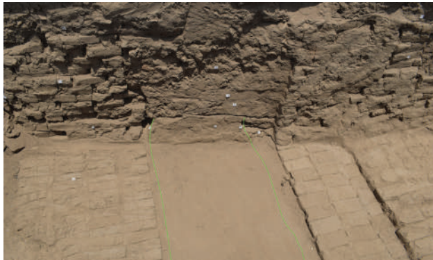
Figure 10: Showing the limits of the foundation trenches and the backfill for the wide wall and the wall to its south. © A. Altaher
