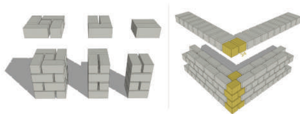
Figure 7: Types of adobe columns found in the Ksar of Timimoun (left). Masonry technique of one adobe/touba (right). © H. Ben Charif
