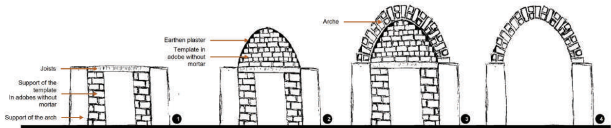
Figure 8: Traditional arches construction in the Ksar of Timimoun. © H. Ben Charif
