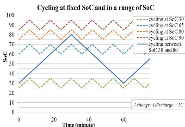
Figure 8 : Difference between cycling at fixed SoC and in a range of SoC
