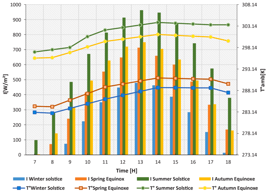
Fig. 9. Daily Fluctuations of the Instantaneous Solar Radiation Intensity and the Ambient Temperature on Four Specific Days of Solstices and Equinoxes in Monastir City.
