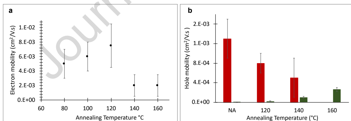
Fig. 6: Charge carrier mobilities measured for composite (PF2:PC 71 BM) (1:2) NPs thin films as a function of annealing temperature (NP diameters = (60 \pm 20) \text{ nm} ). a) Electron mobility measured by SCLC on 140 nm-thick films, b) hole mobility measured by SCLC on 140 nm-thick films (red), and by OFET (green). Each thermal annealing step duration is 10 minutes.
