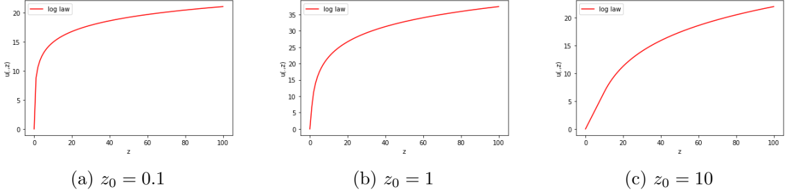
Figure 1: log-law
