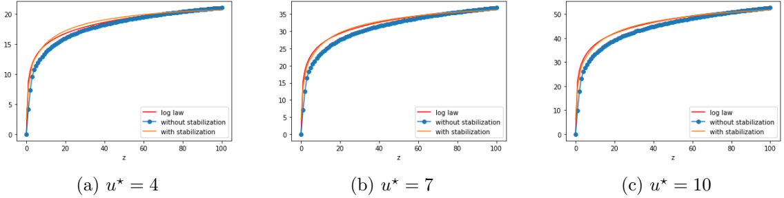
Figure 7: Velocity profile with and without stabilization compared with the log law
