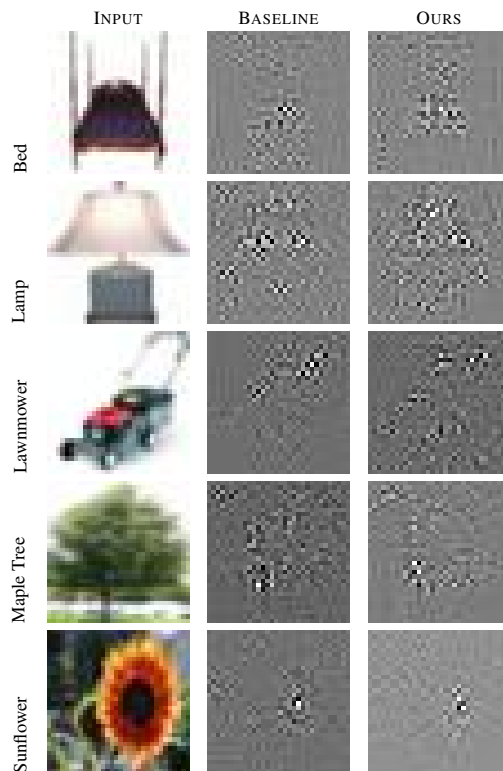
Figure 3: Gradient comparison of standard vs. our training on CIFAR-100 examples.
