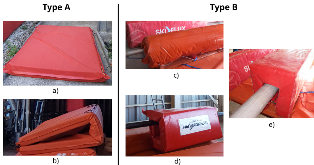
Fig. 1. Left: Type A padding with a) a rectangular shape, and b) a “U” shape, and Right: Type B padding with c) a cylindrical shape, d) a square shape and e) a “U” shape.
