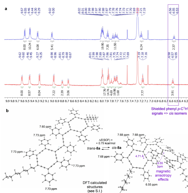
Figure 2. a) Aromatic region of 1 H NMR spectra of the carbo -stilbenes 8a (R = Ph, bottom) and 8b (R = t Bu, top), in CDCl 3 solution (500 MHz, 55 °C). b) DFT-calculated equilibrium structures of cis - 8a and trans - 8a (see Table S4), possibly accounting for magnetic shielding effects on the p -C 1 H nuclei of phenyl substituents made chemically inequivalent by restricted rotation of the C 18 rings with respect to the central DAB connector.
