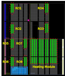
Fig. 3: Methodology to study the effect of the temperatuer generated by our module on ROs frequencies in FPGA.
