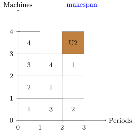
Fig. 4. JSSP with variable unavailability constraints solution obtained.
