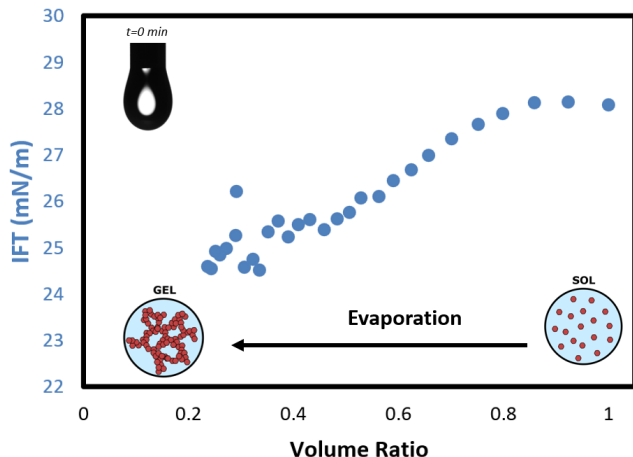
FIG. 8: Surface tension evolution during the sol-gel transition of MTS plotted as a function of the volume ratio defined here as V/V_0 where V_0 is the initial volume of sol
