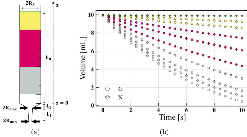
Fig. 1: (a) Schematic representation of the syringe used in the IDDSI flow test and its key dimensions. The initial height of the fluid in the barrel is denoted h_0 and the barrel inner diameter 2R_b . Below the barrel, a cone of length L_2 reduces the inner diameter to 2R_{max} . Finally, a conical nozzle of length L_1 leads to the outlet (diameter 2R_{min} ). (b) Typical evolution with time of the volume of Newtonian liquids in the syringe, measured experimentally. Colours indicate the IDDSI levels obtained from the residual volume at the end of the test
