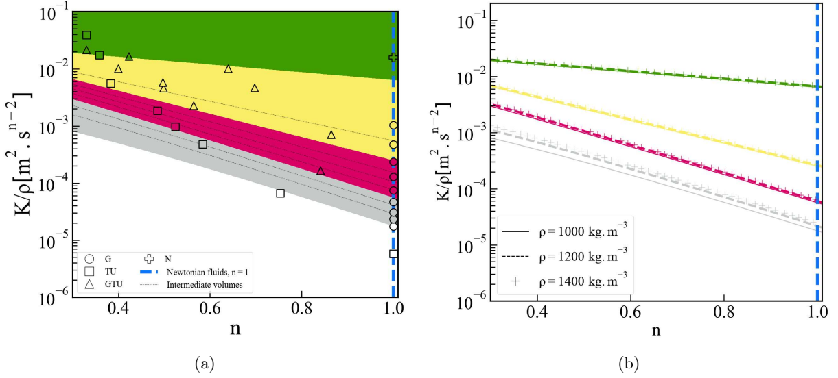
Fig. 6: (a) Rheological map presented in Figure 5 re-scaled by the density \rho . The markers of Level 0 liquids, leaving less than 1mL in the syringe are coloured in white, Level 1 liquids in grey, Level 2 in pink, Level 3 in yellow. (b) The borders of the re-scaled rheological map are not significantly affected by a 20% or 40% increase in fluid density, confirming that the syringe flow test is governed by the kinematic viscosity
