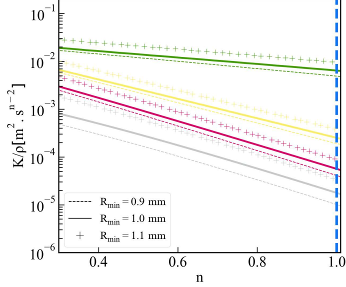
Fig. 7: Effect of a 10% variation of the outlet radius on the borders (solid lines) of the rheological map presented in Figure 5. The grey lines represent the boundary between level 0 and level 1, the pink between level 1 and level 2, yellow between level 2 and level 3, while the green ones represent the upper limits of level 3.
