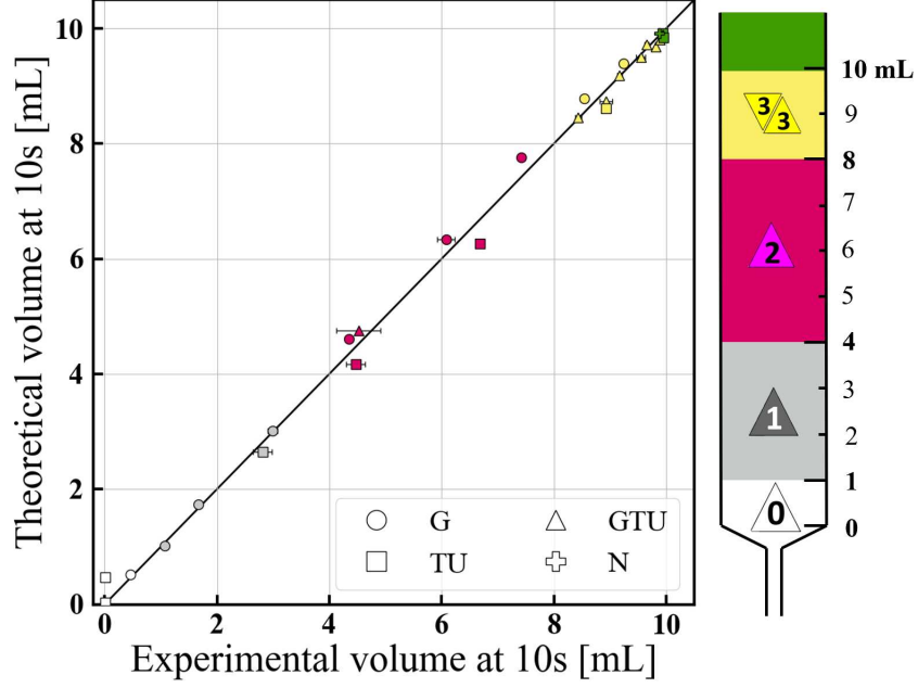
Fig. 4: Volume left in the syringe at 10s: comparison of the theoretical predictions with the experimental measurements. The colours reflect the IDDSI levels. The markers of Level 0 liquids, leaving less than 1mL in the syringe are coloured in white, Level 1 liquids in grey, Level 2 in pink, Level 3 in yellow. The y = x straight line captures the data with R^2 = 0.997 . NB: for some points, the error bars are smaller than the size of the markers
