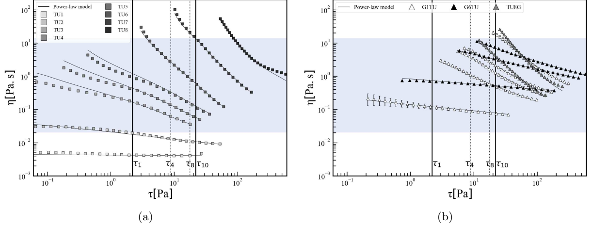
Fig. 2: Viscosity curves of : (a) the aqueous suspensions of TU (compositions indicated in Table 2) (b) the suspensions of TU in glycerol/water solutions, the three GTU formulations are identified by the colour of the marker: white (thickened G1), grey (thickened G6) and black (diluted TU8), see Table 2. The blue-shaded background show the range of viscosity of the Newtonian liquids considered in the study. The vertical solid black lines represent the shear stresses in the nozzle experienced by the fluids throughout the test. The highest stress is labelled \tau_{10} and is caused by the hydrostatic pressure resulting from the initial volume of 10mL of fluid in the syringe, assuming a density of 1000kg/m^3 . The lowest stress is labelled \tau_1 and corresponds to 1mL in the syringe. The intermediate vertical dotted black lines labelled \tau_4 and \tau_8 correspond to a volume of 4mL and 8mL in the syringe, respectively
