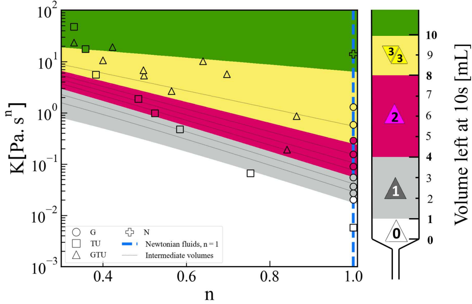
Fig. 5: Rheological map describing the IDDSI levels for a range of the fluid rheological parameters K and n . The regions coloured according to the IDDSI levels are predicted theoretically considering \rho = 1000\text{kg.m}^{-3} , \sigma_{water} = 72\text{mN.m}^{-1} and R_{min} = 1\text{mm} . The vertical dotted line ( n = 1 ) represents the Newtonian fluids, and the dash-dotted lines are the intermediate volumes within each IDDSI levels. The experimental results are also coloured according to the experimental IDDSI level. The markers of Level 0 liquids, leaving less than 1mL in the syringe are coloured in white, Level 1 liquids in grey, Level 2 in pink, Level 3 in yellow. The shape of the mark depends on the type of fluid. The density of the Newtonian fluids used in the experiments differs from \rho = 1000\text{kg.m}^{-3} , which explains some small differences between the level predicted by theory and experiments
