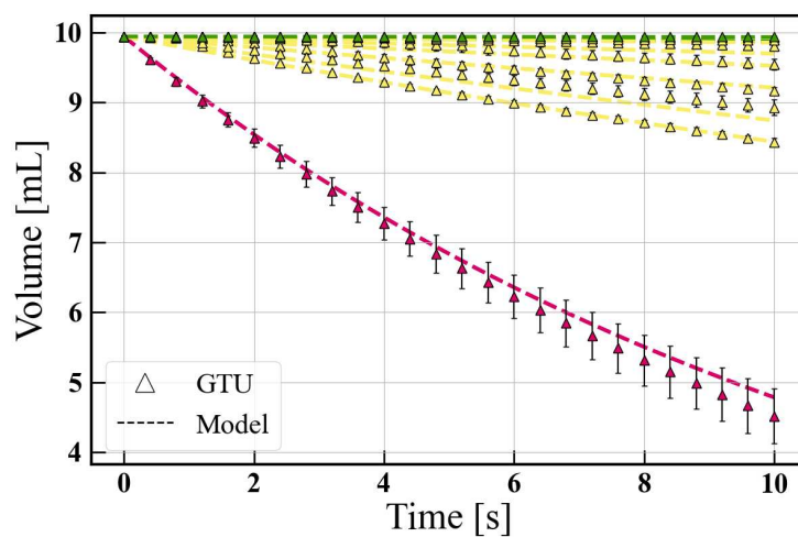
Fig. 8: Evolution with time of the volume left in the syringe for the different GTU solutions considered (presented in Table 2). The marks show the experimental measurements, while the dashed lines show the theoretical predictions. The colours reflect the IDDSI level. A liquid leaving between 0-1mL in the syringe is of level 0 and colored in white, 1-4ml level 1 in grey, 4-8mL level 2 in pink, and 8-10mL level 3 in yellow
