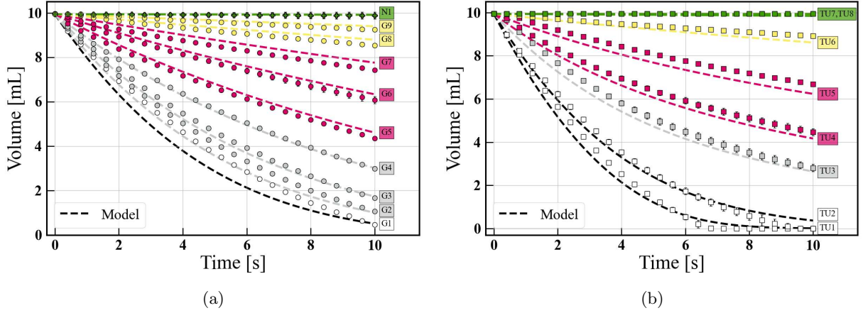
Fig. 3: Evolution with time of the volume left in the syringe for (a) the different Newtonian fluids (b) the different TU solutions considered. The marks show the experimental measurements, while the dashed lines show the theoretical predictions. The colours reflect the IDDSI levels. The markers of Level 0 liquids, leaving less than 1mL in the syringe are coloured in white, Level 1 liquids in grey, Level 2 in pink, Level 3 in yellow
