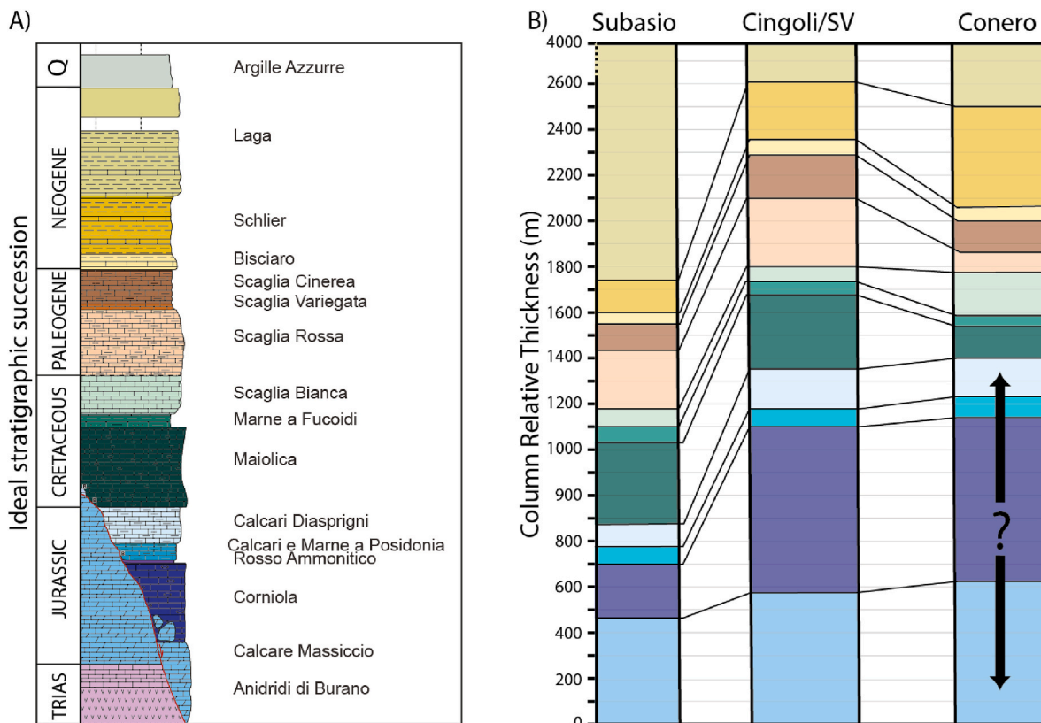
Fig. 3. (A) Ideal stratigraphic column, not to scale, showing the whole Umbria Marche sedimentary succession (in the area of Cingoli Anticline, after Labeur et al. (2021) modified from Petracchini et al. (2012)). (B) Relative overburden of the stratigraphic succession considering the Massiccio Formation as the 0 (bottom) and the Laga Formation as the top. This represents the current stratigraphic thickness of each unit of interest (Jurassic – Paleogene) for the area of the Subasio Anticline (after the geological map, sheet 123 from the Servizio Geologica d'Italia, 1969), the Cingoli/San Vicino pair (after Petracchini et al., 2002) and for the Conero Anticline (after Fancelli and Radrizzani, 1964a, b).
