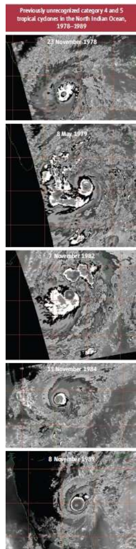
Underestimated storm intensity. The North Indian basin tropical cyclones shown here are listed in the best track data set as category 3 or weaker, but were probably category 4 or 5. Similar underestimates may have been common in all ocean basins in the 1970s and 1980s. Trend analyses for tropical cyclones intensities are therefore highly problematic.
