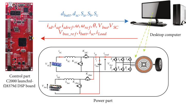
FIGURE 14: PIL cosimulation strategy scheme.
