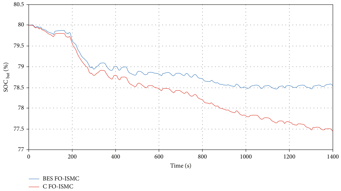
FIGURE 9: Battery state of charge (%).
