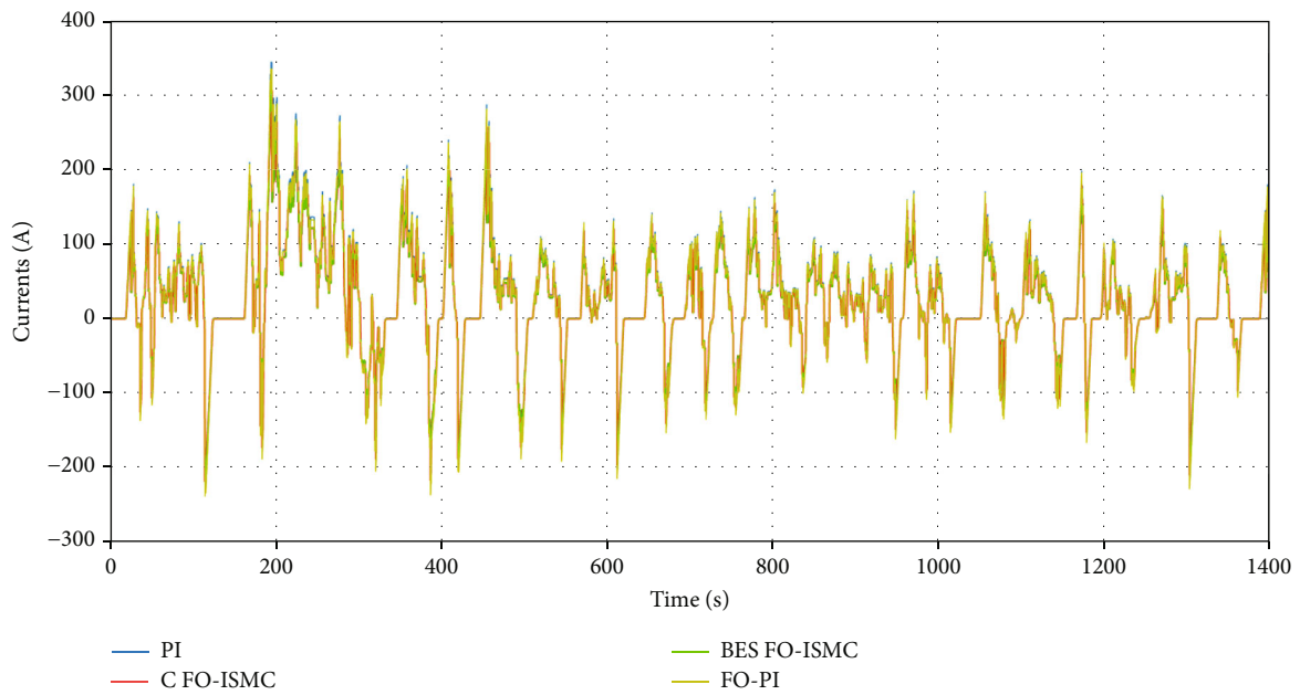
FIGURE 10: Battery current.
