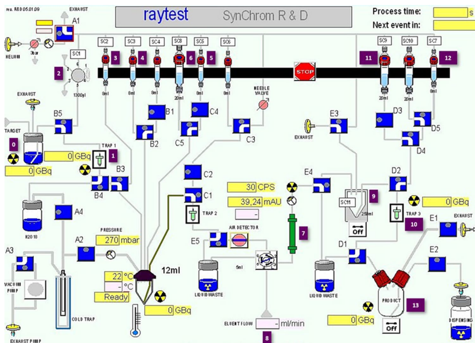
Scheme 1 Raytest SynChrom R&D Evo I layout for the automated production of (S)-[ 18 F]FETp from precursor (S)-3. 0: aqueous solution of [ 18 F]fluoride in [ 18 O]H 2 O; 1: anion exchange Sep-Pak® QMA cartridge (46 mg); 2: solution of TBA-HCO 3 (4.4 mg, 14.5 μmol) in H 2 O/MeCN (1 mL, 1/1, v/v); 3: anhyd. MeCN (2 mL); 4: precursor (S)-3 (2 mg) in anhyd. DMF/t-BuOH, (1 mL, 9/1, v/v); 5: 6 M aqueous HBr solution (500 μL); 6: 1.1 M NaOAc buffer solution pH 5.5 (3.5 mL); 7: Symmetryprep C18 column (300 × 7.8 mm; 7 μm; Waters); 8: H 2 O/MeCN/TFA (90/10/0.01, v/v/v), isocratic mode, λ = 254 nm, flow rate = 1.5 mL/min for one min and then 2.5 mL/min; 9: collection vial pre-filled with deionised H 2 O (20 mL); 10: pre-conditioned Oasis MCX plus short cartridge; 11: deionised H 2 O (10 mL); 12: 5% NH 4 OH/EtOH solution (3 mL); 13: final product vial for formulation with saline (30 mL) and AcOH (135 μL)
