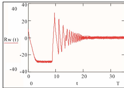
Figure 17. Speed of rapprochement missile-to-target: \dot{R}(t) .
