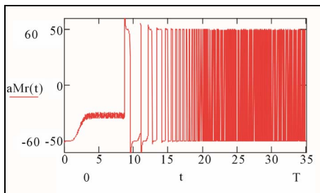
Figure 21. Missile acceleration along target-to-missile direction: a_M^n(t) .
