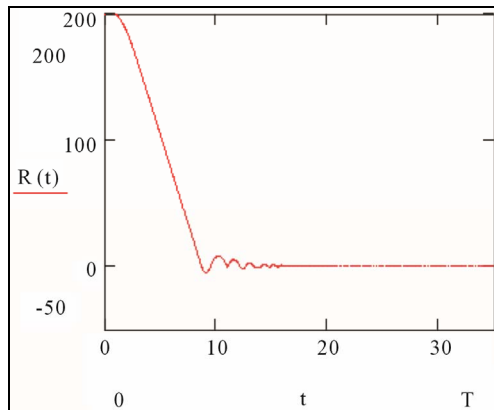
Figure 16. Target-to-missile range R(t) . R(t) = 7.2 \times 10^{-3} m.
