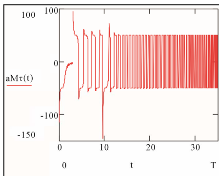
Figure 22. Missile acceleration along direction which perpendicularly to line-of-sight direction: a_M^n(t) .
