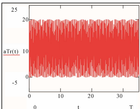
Figure 23. Target acceleration along target-to-missile direction: a_r^n(t) .
