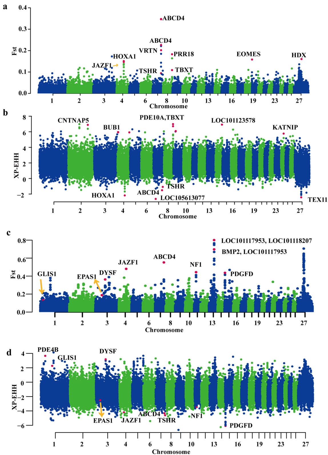
Fig. 3 Positive selection scans for adaptation to drought and high-altitude conditions. Fst and XP-EHH for 50-kb windows are plotted along the ovine whole genome. Chromosomes are represented by color. Genomic landscape of the Fst values ( a ) and XP-EHH values ( b ) in the genome of sheep breeds from drought areas. Genomic landscape of the Fst values ( c ) and XP-EHH values ( d ) in the genome of sheep breeds from high-altitude areas
