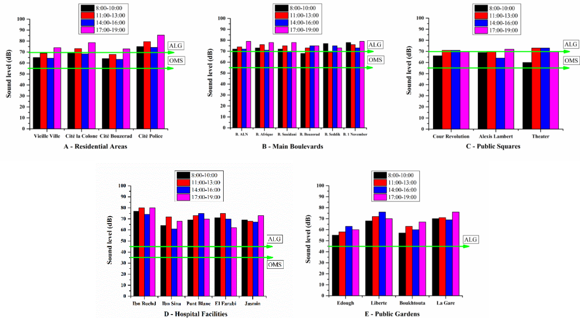
Figure (N°2). Averaged Leq_{max} at the five selected areas in Annaba city
