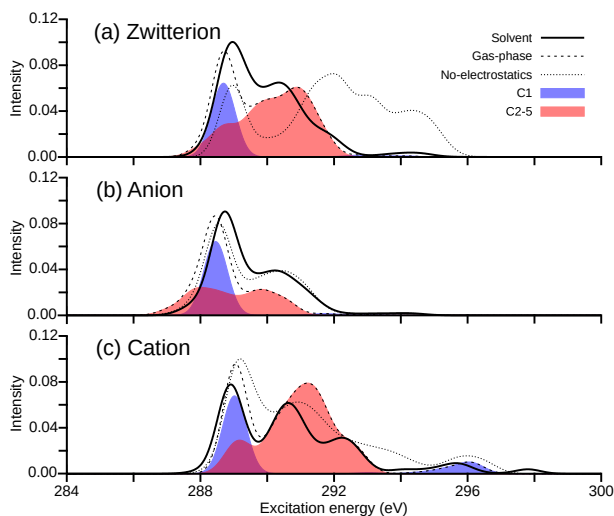
Figure 6: Carbon K-edge absorption of (a) zwitterionic, (b) anionic, and (c) cationic in solution (solid line), gas phase (dashed), and no electrostatics (dotted). The gas phase XAS spectrum comes along with its analysis (shaded area) and corresponds to carbon 1 (blue) and carbon 2 to 5 (red) according to the nomenclature of Fig. 2. The spectra for the solvent model converged up to 296.43, 294.97, and 297.98 eV for the zwitterionic, anionic, and cationic structures, respectively.
