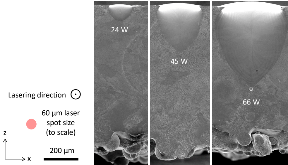
Fig. 4: BSE images showing the melt pool depths at the sample edge after lasering with s 60 \mu\text{m} , v 50 \text{ mm/s} and varying P (second parametric study).
