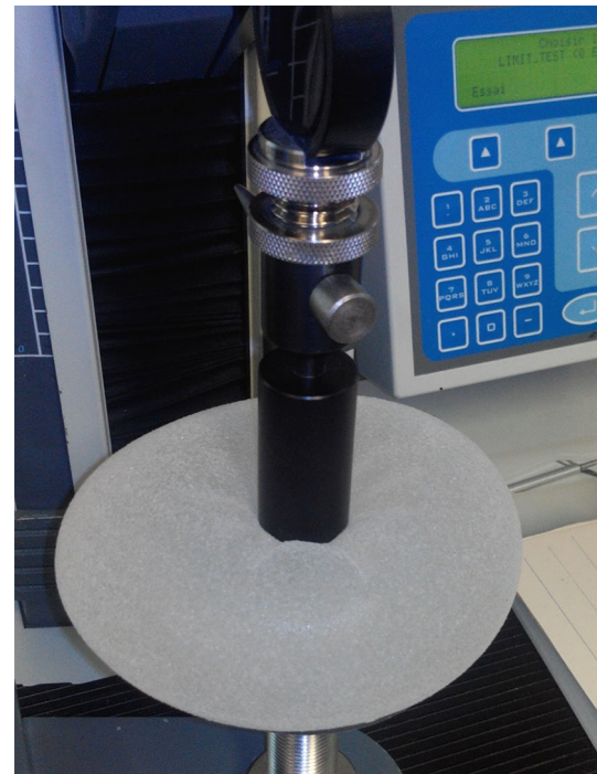
Fig. 1 Implants stiffness test
