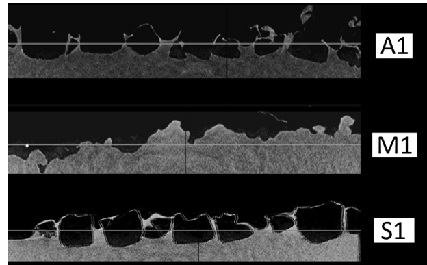
Fig. 3 X-ray microtomography images of A1, M1, and S1 shells
