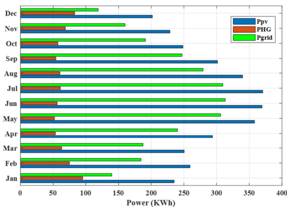
Fig. 7. Annual power generation from the PV system, grid supply, and hydroponic greenhouse power demand.
