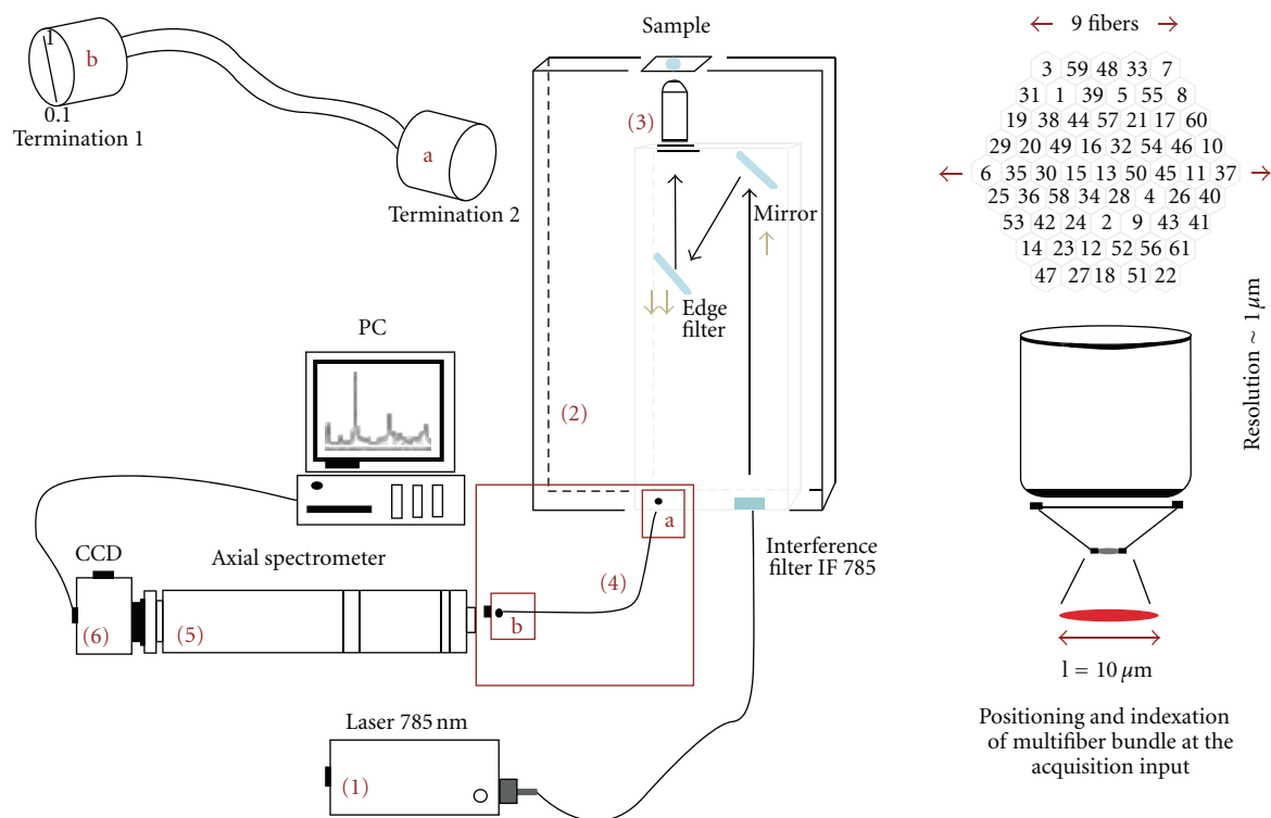
FIGURE 1: Schematic view of the Raman imaging probe setup.
