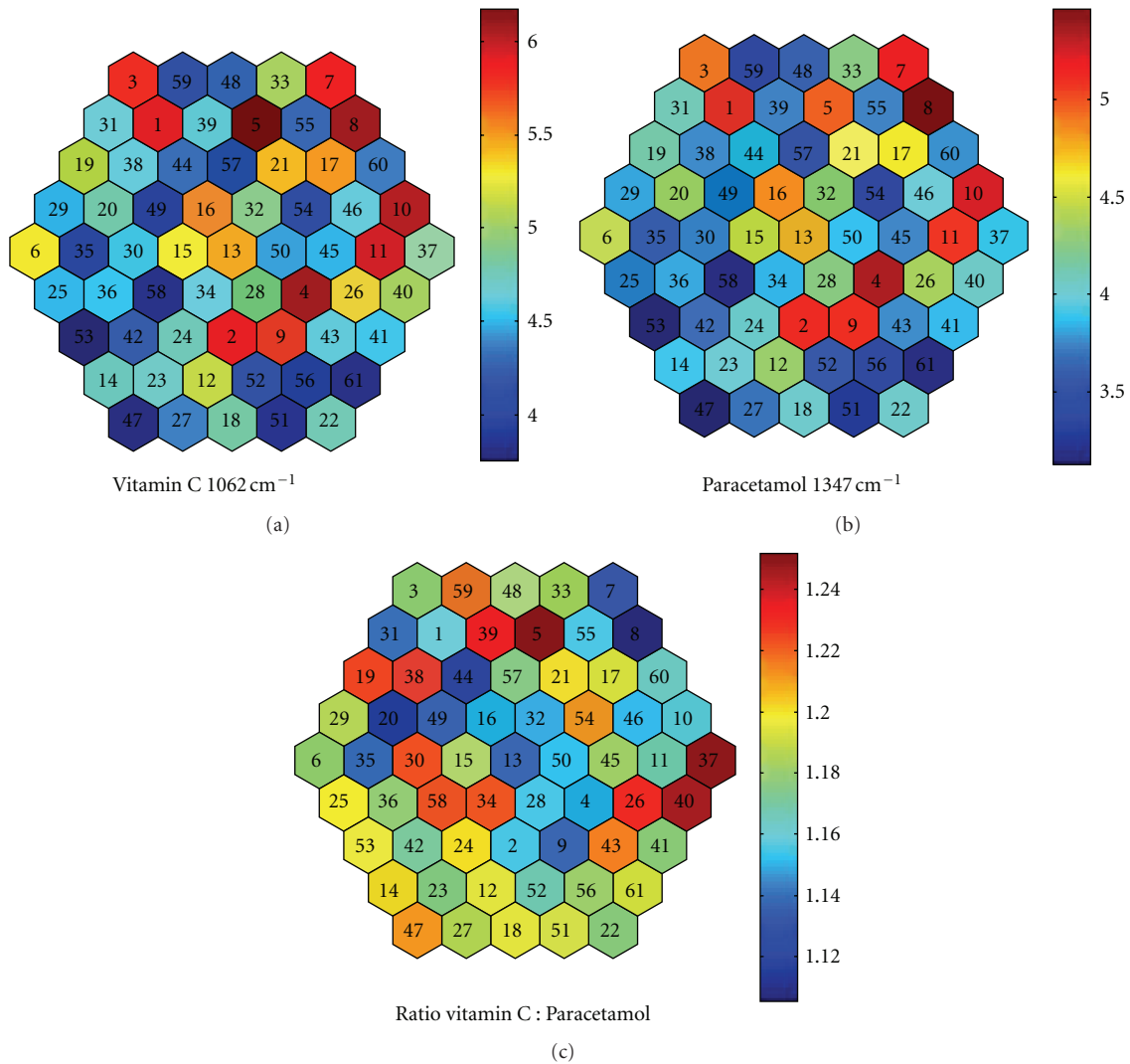
FIGURE 5: Constructed images showing the distribution of vitamin C (a) and paracetamol (b) within the Efferalgan tablet. Distribution ratio is displayed in (c). The color code bars represent intensity variations (a.u.) of the respective vibrations.
