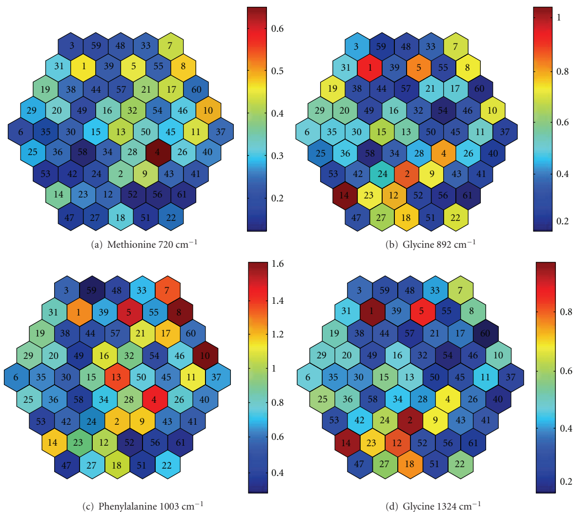
FIGURE 4: Constructed images showing the distribution of methionine (a), glycine ((b) and (d)), and phenylalanine (c) within the tri-amino-acid pellet. The color code bars represent intensity variations (a.u.) of the respective vibrations.
