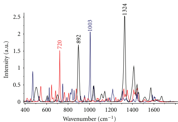
FIGURE 2: Raman spectra of phenylalanine, methionine, and glycine. Specific vibrations used for the detection of each of the 3 amino-acids are indicated.
