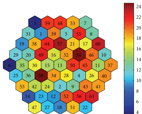
FIGURE 3: Fibre response image constructed from silicon Raman vibration at 520 \text{ cm}^{-1} . The color code bar represents intensity variation (a.u.) of the vibration.
