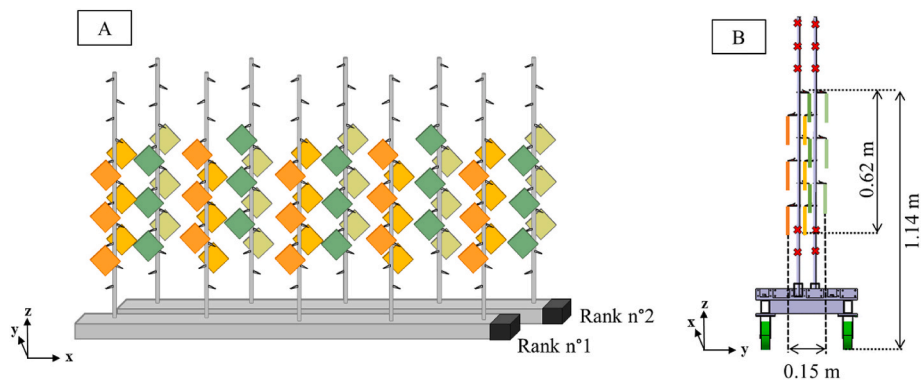
Fig. 5. Side view (A) and cross-sectional view (B) of the EvaSprayViti collection compartments at early-stage vegetation. The different colours distinguish the four compartments defined by depth. The red crosses symbolise positions where collectors have not been positioned. Measurements provided are indicative. For convenience of graphics, only half of the poles are represented on the side view. (For interpretation of the references to colour in this figure legend, the reader is referred to the Web version of this article.)
