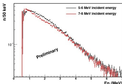
Figure 4. Preliminary ^{235}\text{U}(n,f) PFNS for 5 to 6 and 7 to 8 MeV incident energy bins. Only a part of the statistics is presented.
