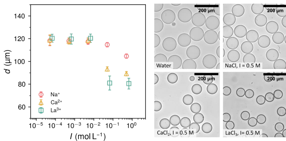
Figure S 4: Swelling behavior of hydrolyzed particles (HP60) in the presence of NaCl, CaCl 2 , and LaCl 3 . (Left) Particle diameter ( d ) as a function of ionic strength ( I ). (Right) Microscopy images of HP60 particle suspensions in water, and in the presence of NaCl, CaCl 2 , and LaCl 3 at I = 0.5 M.
