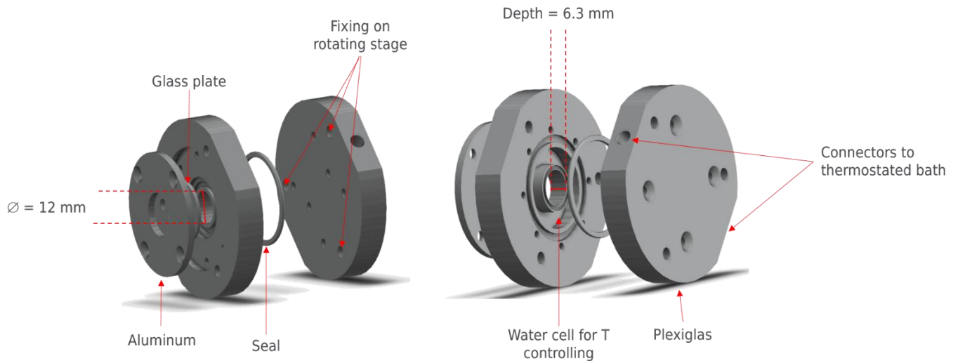
Figure S 2: Schematic of the thermostatically controlled drum used for temperature-varying experiments. The drum is connected to a thermostated bath and a peristaltic pump to control the temperature and water flow around the drum cell.
