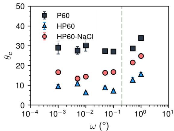
Figure S 3: Avalanche angle ( \theta_c ) as a function of rotation speed ( \omega ) for poly(methyl methacrylate) (PMMA) particles (P60) in pure water and hydrolyzed poly(sodium methacrylate) (PMAA-Na) particles (HP60) in pure water and in presence of NaCl ( I = 0.5 M). For \omega \leq 0.2 ^{\circ}.s^{-1} , the avalanche angle ( \theta_c ) is independent of \omega , i.e. measurements are performed in a quasi static regime.
