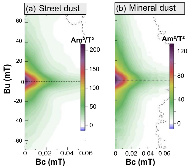
Figure 5. FORC diagrams for resuspension products: (a) street dust, and (b) mineral dust.
