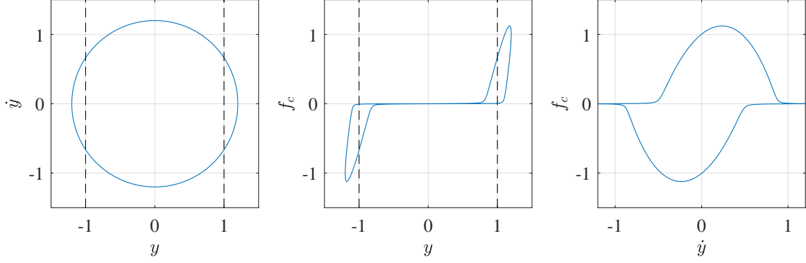
Figure 1: Illustration of the smooth impact function, with an assumed periodic displacement y(t) = 1.2 \cos(2\pi t) and parameters: k_c = 5 , c_c = 1 , g_k = 1 , \eta = 10^{-4} . Dashed lines represent the contact locations.
