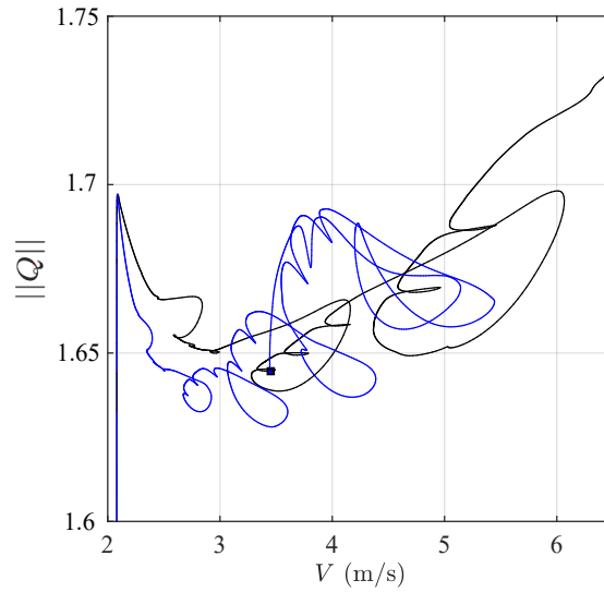
Figure 11: Continuation of periodic solutions for three-mode model. Black: symmetric branch; blue: asymmetric branch. ■ BP
