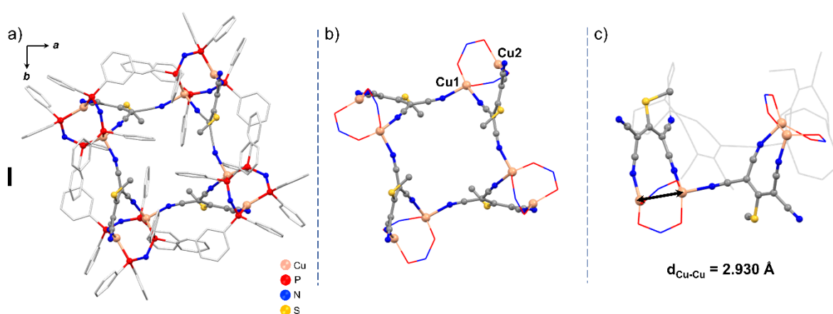
Figure 3. Molecular X-ray structure of derivative I . a) General view from the ‘top’ of the metallacycle and simplified views (phenyl rings have been omitted for clarity) from b) the ‘top’ and c) the side of the metallacycle.
