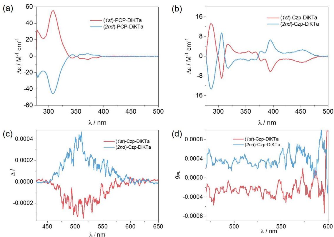
Figure 5. Experimental ECD spectra of (a) (1st)/(2nd) -PCP-DiKTa and (b) (1st)/(2nd) -Czp-DiKTa in toluene. Experimental CPL spectra (c) and g_{PL} values (d) of (1st)/(2nd) -Czp-DiKTa in toluene ( \lambda_{exc} = 444 nm). (1st)/(2nd) -enantiomers refer to the 1 st and 2 nd enantiomers eluted by chiral HPLC.
