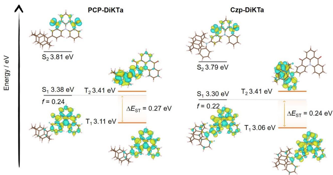
Figure 2. Difference density plots and energies for the S 1 , S 2 , T 1 and T 2 of PCP-DiKTa and Czp-DiKTa calculated at SCS-CC2/cc-pVDZ in the gas phase (ISO value = 0.02). The blue color represents an area of decreasing electron density, and the yellow color represents an increased electron density between the ground and excited states.
