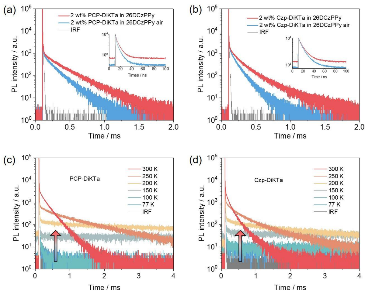
Figure 4. Time-resolved PL decays ( \lambda_{\text{exc}} = 343 nm) of (a) PCP-DiKTa and (b) Czp-DiKTa in 2 wt% doped film in 26DCzPPy (inset figures are the time-resolved PL decays of the prompt component, \lambda_{\text{exc}} = 375 nm). Temperature-dependent time-resolved PL decay of (c) PCP-DiKTa and (d) Czp-DiKTa in 2 wt% doped film in 26DCzPPy, \lambda_{\text{exc}} = 343 nm.
