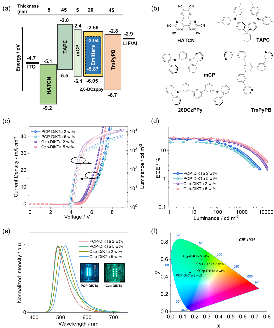
Figure 5. (a) Schematic of the OLED stack; (b) Chemical structures of the materials used in the device; (c) Current density-voltage-luminescence (JVL) characteristics; (d) External quantum efficiency (EQE) vs luminance; (e) Electroluminescence spectra, inset figures are photographs of the OLEDs fabricated with PCP-DiKTA 2 wt% and Czp-DiKTA 2 wt% ; (f) CIE coordinates of the devices.
