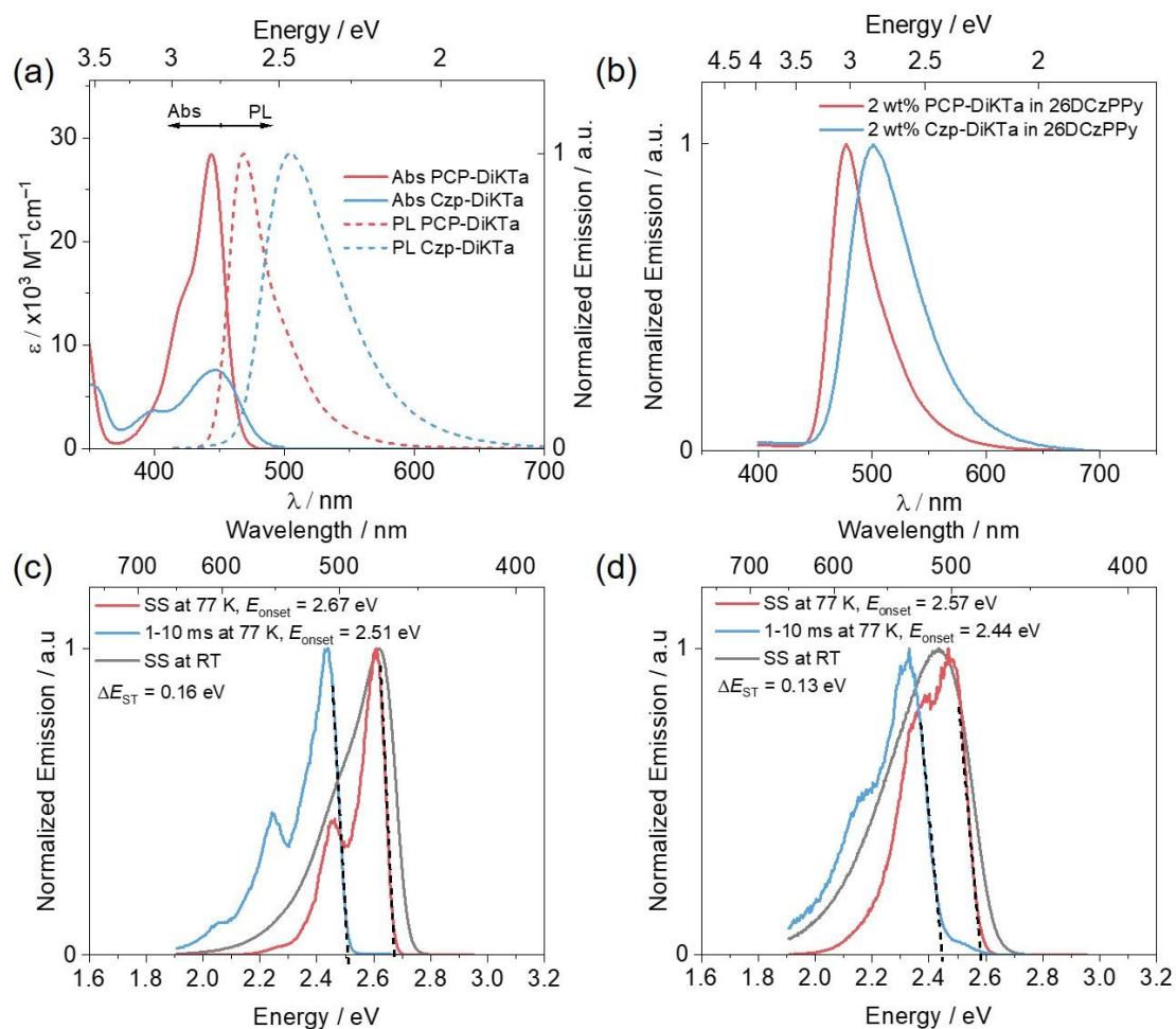
Figure 3. (a) UV-vis absorption and steady-state PL spectra recorded in aerated toluene at 298 K ( \lambda_{exc} = 340 nm). (b) Steady-state PL spectra ( \lambda_{exc} = 343 nm) in 2 wt% doped films. (c) Steady-state PL spectra of PCP-DiKTa at 77 K and room temperature ( \lambda_{exc} = 353 nm), and phosphorescence spectra at 77 K (1-10 ms, \lambda_{exc} = 353 nm) in toluene. (d) Steady-state PL spectra of Czp-DiKTa at 77 K and room temperature ( \lambda_{exc} = 365 nm), and phosphorescence spectra at 77 K (1-10 ms, \lambda_{exc} = 365 nm) in toluene; concentration: 1 \times 10^{-5} M.
