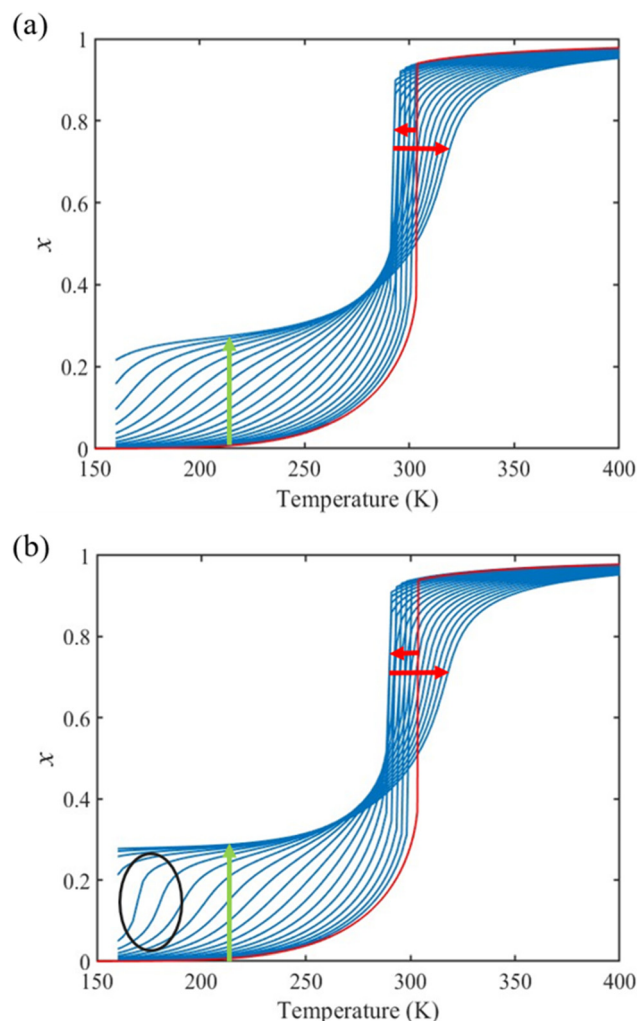
Fig. 4 Calculated temperature dependence of the HS fraction (heating mode) in a 5 nm thin film of [Fe(pyzriline)][Ni(CN) 4 ] in the case of (a) \alpha = \frac{\sigma_{\text{LS}}}{\sigma_{\text{HS}}} = 1.4 and (b) \alpha = \frac{\sigma_{\text{LS}}}{\sigma_{\text{HS}}} = 2.0 for different positive values of \sigma_{\text{HS}} ranging from +10 to +410 \text{mJ m}^{-2} with an increment of 20 \text{mJ m}^{-2} . The red curve represents the bulk material. Green and red arrows are guides for the eye to follow the evolution of the residual HS fraction and the equilibrium temperature, respectively, with increasing values of \sigma_{\text{HS}} . The black circle highlights an abrupt spin transition in the shell brought into by the tensile stress.
