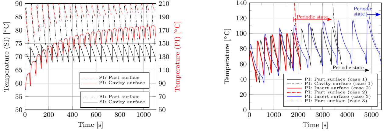
(a) Steel and plastic inserts cases: default IM parameters.
